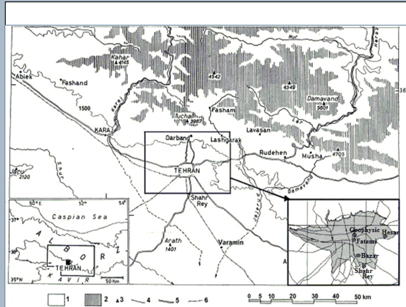
Fig.1: The situation of air pollution stations in city of Tehran. The numbers show 1: regions of altitude less than 1500 m a.s.l., 2: altitude ranges of 1500-3000 m a.s.l., 3: summit of mountain, 4: river, 5: highway, and 6: railway.
