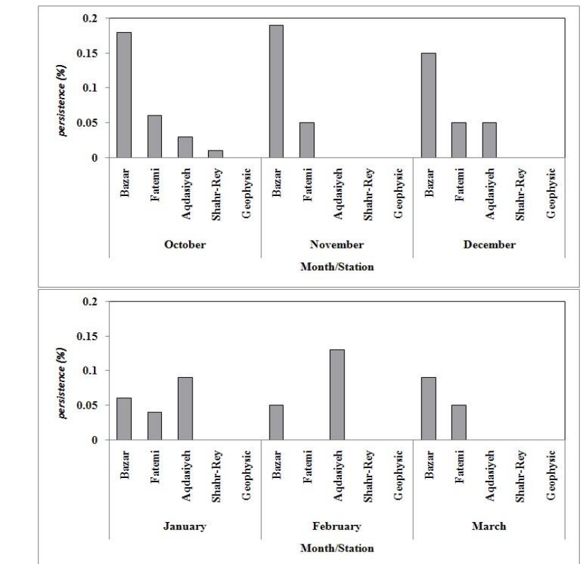
Fig.2: persistence of days along with PM10 pollutant at different months of the year in stations of interest.
