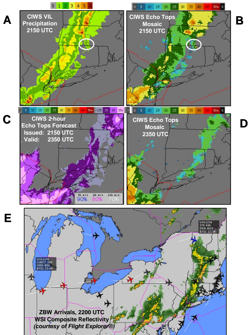
Figure 9: (A) CIWS NEXRAD VIL Precipitation on 6 June 2005 at 2150 UTC, (B) CIWS Echo Tops Mosaic at 2150 UTC, (C) CIWS 2-hour Echo Tops Forecast issued at 2150 UTC, (D) CIWS Echo Tops Mosaic at 2350 UTC, time of Echo Tops Forecast verification, and (E) FlightExplorer® flight tracks and Weather Services Inc. (WSI) composite reflectivity showing flights en route to Boston (MA), Providence (RI), Hartford (CT), and Manchester (NH) airports. At 2150 UTC, a near solid line of level 3+ convection, with embedded echo tops exceeding 30 kft, continued to significantly impact air traffic operations in the Boston (ZBW) ARTCC (see A and B). Despite near-term storm severity, and the threat of new storm development (circled region in A and B) ZBW traffic managers used the 2-hour Echo Tops Forecast (see C) and the looping past Echo Top Mosaic to determine that storm heights were decreasing and key airways blocked by weather would be available to ease capacity constraints. Forecast accuracy scores for predicting 30 kft+ echo tops at 30, 60, and 120 min were 90%, 80%, and 70%, respectively (See C – inset). Using this Echo Tops Forecast, ZBW traffic managers, in collaboration with neighboring ARTCCs, allowed en route transcontinental flights to ZBW (see E – aircraft colored red) to discontinue longer, more complex reroutes around the north end of the squall line (see E – aircraft colored blue in northern VT is last flight to use extended reroute) and return to normal routes through central NY. Additionally, the ground stop for Chicago O’Hare (ORD) flights to ZBW airports was discontinued early based upon the Echo Tops Forecast (see E – flight departing from ORD to Hartford). Inspection of the Echo Tops Mosaic at the time of forecast verification (See C and D) demonstrates the accuracy of the 2-hour Echo Tops Forecast.
