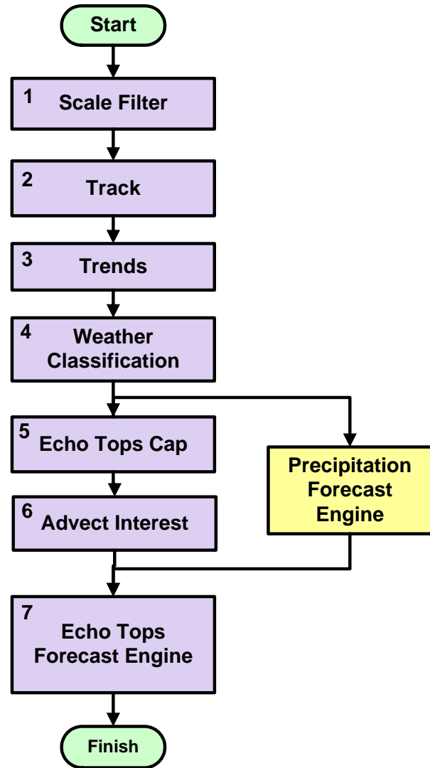
Figure 2: The functional flow of the ETF algorithm. The purple boxes represent the main components of the ETF algorithm. The yellow box depicts the generation of the precipitation VIL forecast. Note: The first four steps (Scale Filter, Track, Trends, and Weather Classification) are also steps in the generation of the precipitation VIL forecast but for simplicity the details are not depicted in this diagram.
