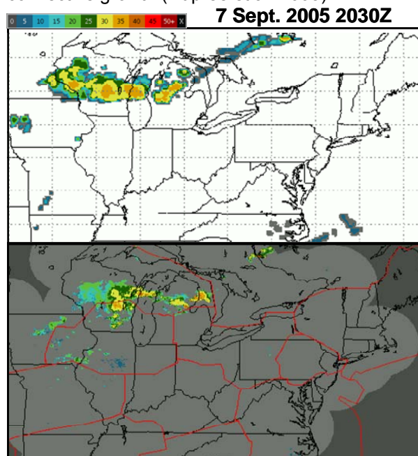
Figure 12: MM5 Echo Tops Forecast: Shown are the 8.5 hour lead time MM5-generated Echo Top Forecast in kft (top) and the CIWS Echo Tops Mosaic in kft at the time of forecast validation (bottom). The spatial resolutions are 9 km and 1 km for the MM5 ETF and the Echo Tops Mosaic respectively.
