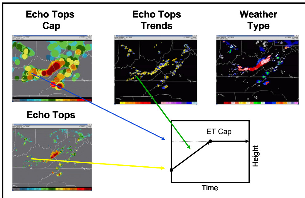
Figure 6: Echo Tops Forecast Engine. The echo tops forecast engine applies a simple growth model to the current echo tops height field. Short-term echo tops growth rates are applied as a function of forecast time horizon in regions of convective weather, until the echo top height reaches the maximum cap as measured by previous echo tops distributions in the area. Non-convective weather is simply advected and growth and decay trends are not used.
