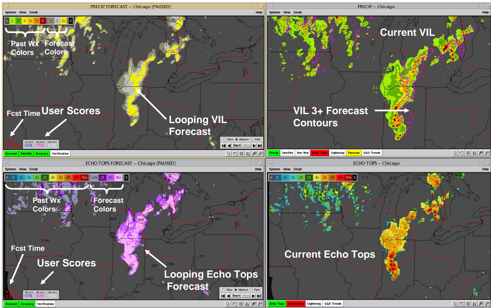
Figure 1: Display of Precipitation, Echo Tops, and 0-2 hour Forecasts of Precipitation and Echo Tops on CIWS Situation Display: The upper left window is the looping VIL Forecast. The lower left is the looping Echo Tops Forecast. The upper right is the current VIL with the 60 minute forecast level 3 contours overlay. The lower right is the current Echo Tops Mosaic.
