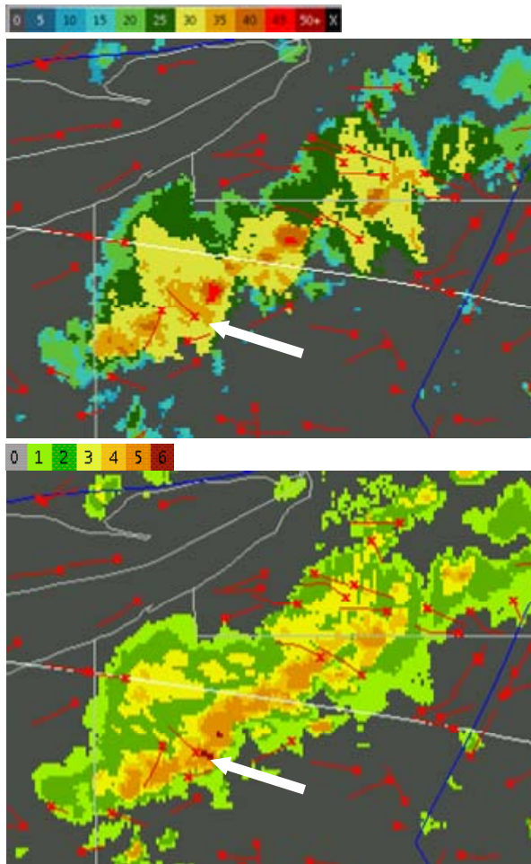
Figure 10: Echo Tops Mosaic in kft (top) and 6-level VIL precipitation (bottom). The red 'x' and tail denotes flight tracks \geq 16 kft. The white arrows show an area where planes are flying in the vicinity high tops ( >35 kft) and high VIL ( \geq level 3). This figure demonstrates that depictions of high tops ( >35 kft) and high VIL ( \geq level 3) are not necessarily adequate indicators of no-fly zones as shown in the ETFs and PFs.
