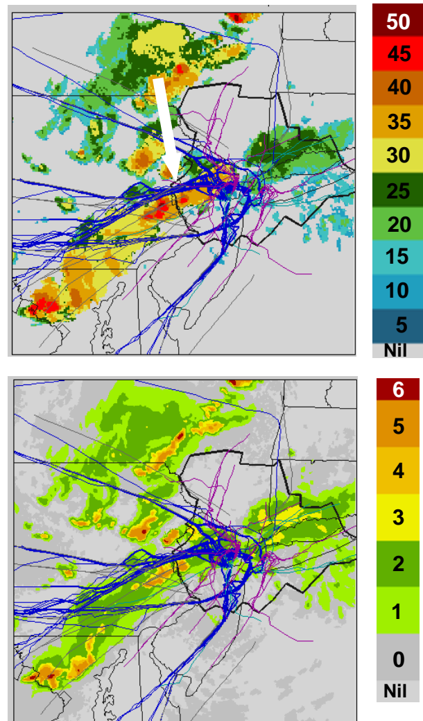
Figure 11: This figure shows Echo Tops in kft in the top image and 6-level VIL in the bottom with cumulative departures (dark blue and cyan) and arrivals (magenta) in New York Terminal Radar Approach Control (TRACON) (heavy black line) over a 30 minute period centered on 2245Z on June 29, 2005. Note westbound traffic flow around 50 kft convective cell (white arrow) on the TRACON boundary, where aircraft are still climbing to cruise altitudes.
