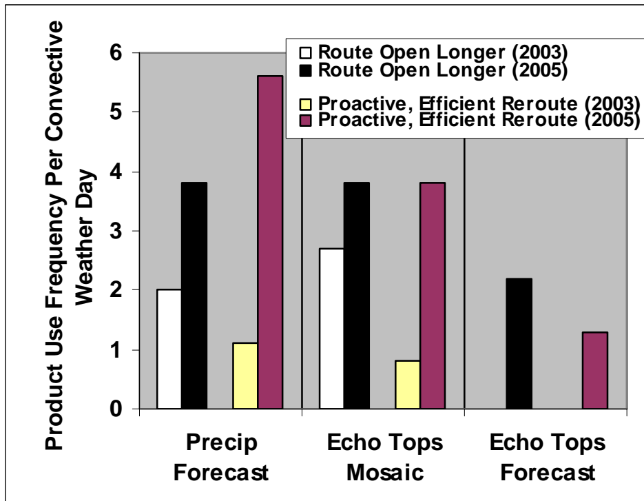
Figure 8: Frequency of CIWS Forecasts and Echo Tops Mosaic usage in 2003 versus 2005 to achieve two primary CIWS en route air traffic delay reduction and airspace complexity benefits: Keeping Routes Open Longer and More Proactive, Efficient Reroutes.
