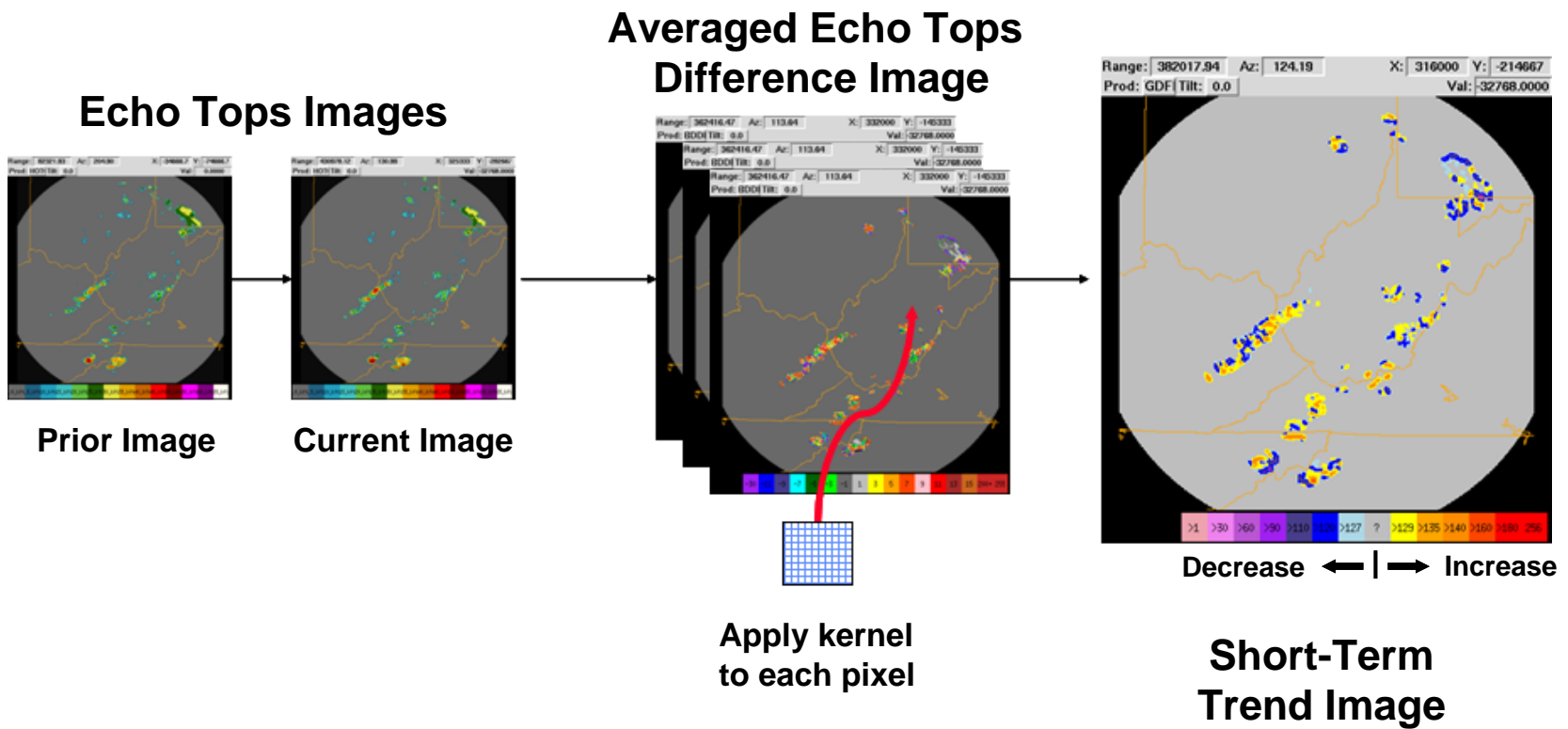
Figure 4: Echo Tops Trends: This figure shows the algorithm steps used to create the echo tops short-term growth and decay interest. The first step shows the differencing of prior images, the middle graphic is the step where previous images are temporally and spatially averaged, the right image is the final short-term echo tops growth and decay image.
