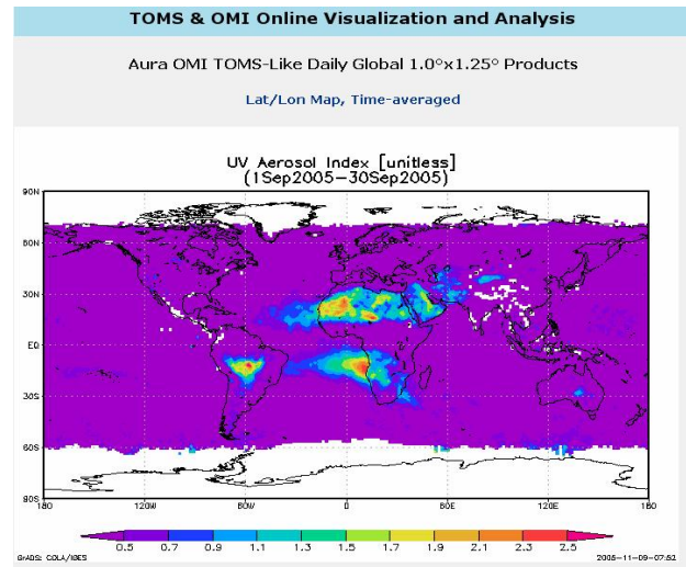
Fig 2a - Global distribution of Dust and smoke (OMI Aerosol index averaged for September 2005)
