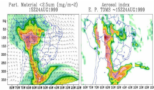
Fig.1 PM2.5 forecast and TOMS Aerosol index over Chile, South America (source: S. R. Freitas et al., http://www.fire.unifreiburg.de/vfe/vfe_southamerica.htm )
