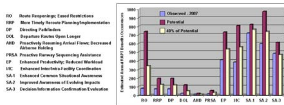
Figure 8. Estimates of the annual frequency of RAPT benefits for observed usage in 2007, full, near-term potential usage, and 40% of full potential RAPT usage.
