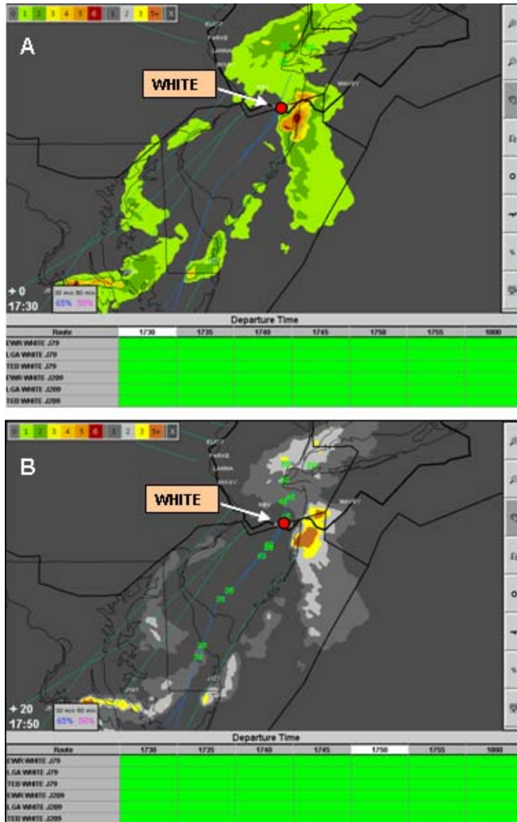
Figure A-1-4-1. RAP T guidance at 1730 UTC on 16 August 2007 showing (A) a strong storm just east of the WHITE departure fix and (B) the 20-min forecast showing the level 5+ thunderstorms moving eastward and away from the WHITE route. RAP T timelines for WHITE departure routes from all NY airports correctly predicted that significant weather would clear the route and that the route would remain viable for the foreseeable future.
