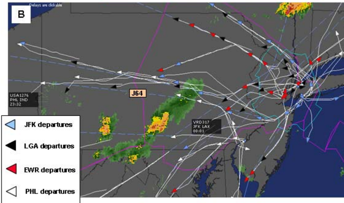
Figure A-3-2-1. (A) RAPT guidance at 2335 UTC on 30 August 2007 predicting weather blockages by high echo top precipitation becoming less severe for departures at 2345 UTC and beyond (see boxed timeline). (B) Flight Explorer flight tracks and WSI composite reflectivity at 0020 UTC showing the PHL (white) and JFK (blue) pathfinders (flights tagged with departure information) airborne and testing the route at this time.
