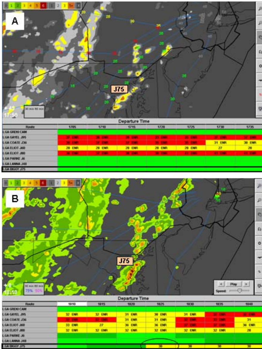
Figure A-4-1-1. RAP T guidance at (A) 1705 UTC and (B) 1810 UTC on 11 July 2007. At 1705 UTC, a cluster of storms was developing in southeast PA, but RAP T showed that J75, through this region, was unblocked by weather (in box in (A)) LGA traffic managers used this information to argue against a route closure and to keep the J75 departure route open. The cluster of storms slowly intensified and eventually caused pilot deviations large enough to close J75 at 1825 UTC. RAP T guidance at 1810 UTC correctly anticipated that conditions for J75 departures would deteriorate starting with 1825 UTC departures (circled). Note yellow timeline which indicates partial blockage or “caution”.
