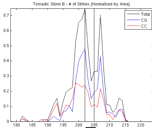
Figure 22: CC and CG flash rates for the EF2 tornadic cell on March 15th
