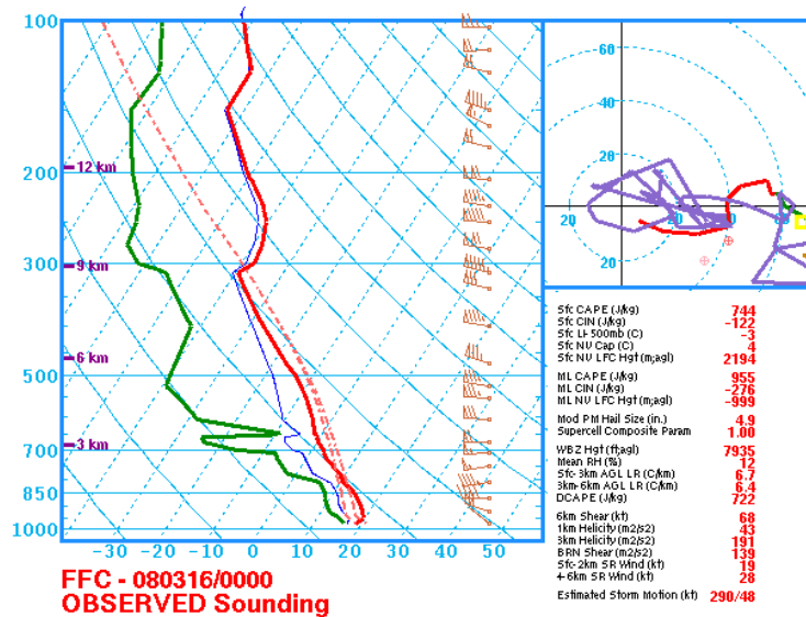
Figure 13: Skew-T Diagram for 00Z March 16th
