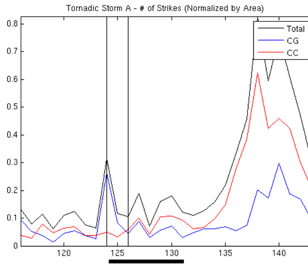
Figure 19: Total flashes (CC + CG) for EF3 cell with area normalization.
