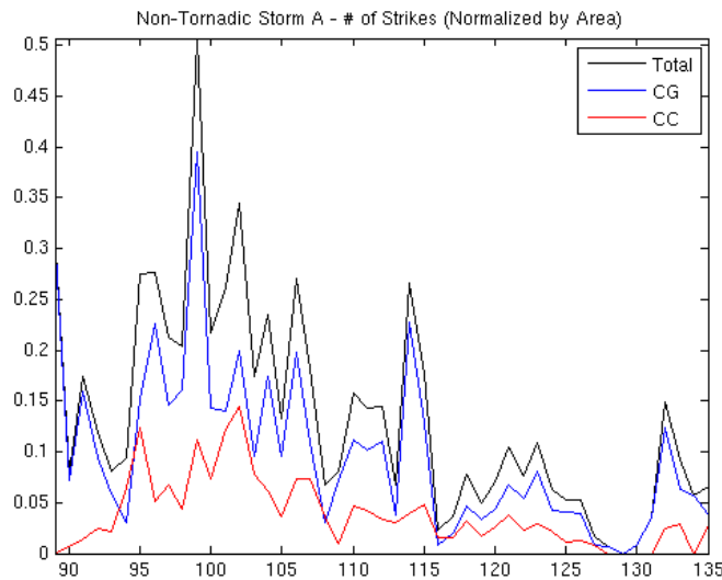
Figure 20: Normalized CC and CG Flash Rates for first non-tornadoic cell on March 15th
