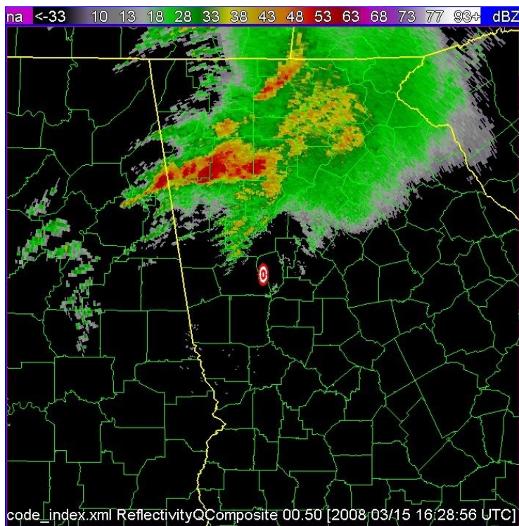
Figure 14: NEXRAD composite reflectivity at 16:29 UTC on March 15th
