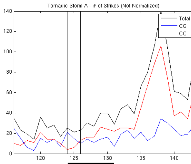
Figure 18: Total flashes (CC + CG) for EF3 tornadic storm without area normalization.
