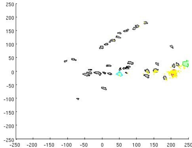
Figure 17: DBSCAN SCITs and associated NLDN flashes at 22:15 UTC on March 15th.
