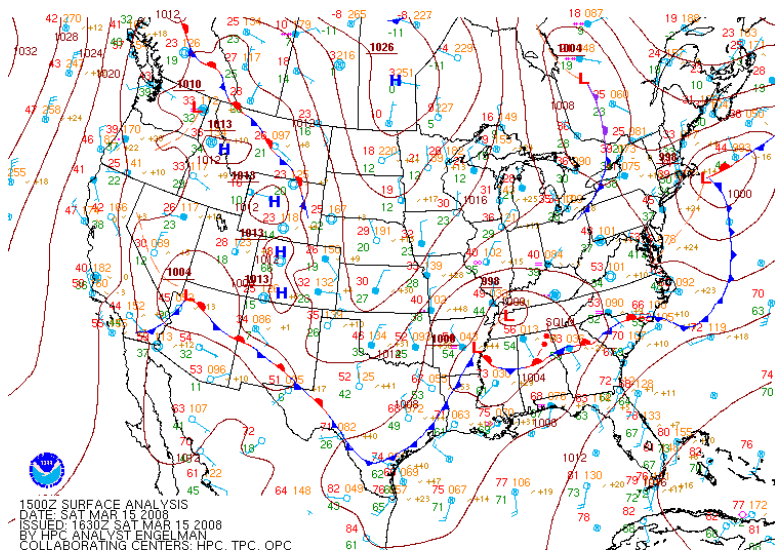
Figure 10: Surface Chart for 15Z on March 15th.
