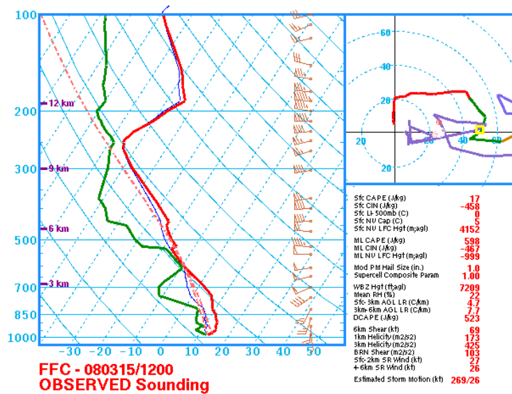
Figure 12: Skew-T Diagram for 12Z on March 15th.
