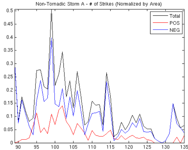
Figure 21: Normalized Positive and Negative flash rates for first non-tornadic cell studied on March 15th.
