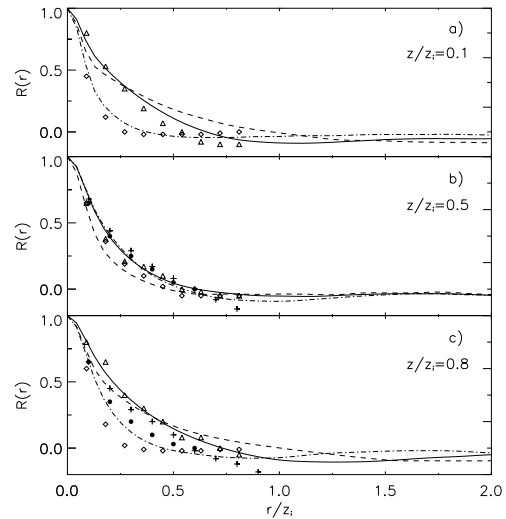
FIG. 1: Eulerian autocorrelation function R^E(r) calculated at different heights as a function of the normalized space lag r/z_i . Continuous line: u -component, dashed line: v -component, dashed-dotted line: w -component. The following numerical and experimental data are also shown: diamonds and triangles, Mason (1989); circles and +, Deardorff and Willis (1985).
