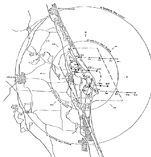
Fig. 10. First Thunderstorm Overlay.
