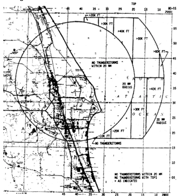
Fig. 11. First Thunderstorm Keyhole (NASA, 1989).
