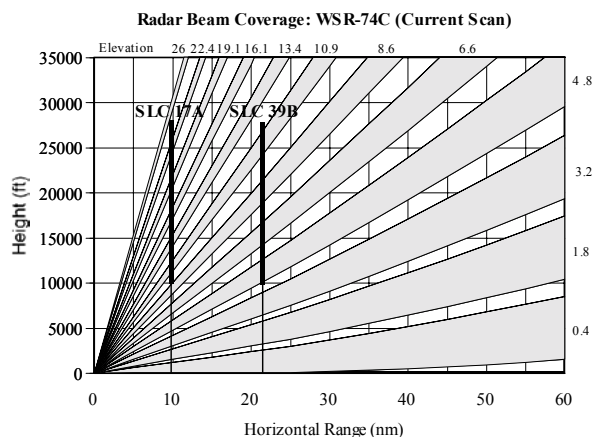
Fig. 8. Radar Scan Strategy.
