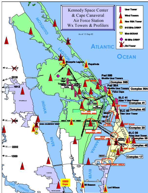
Fig. 7. Weather Instrumentation.
