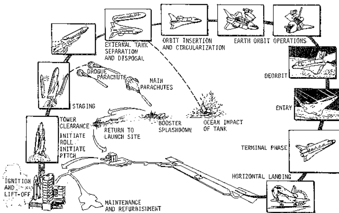
Fig. 9. Typical Shuttle Mission Profile (NASA, 1977).
