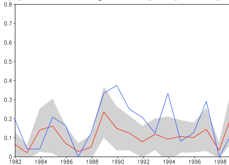
(a) Alaskan Ridge NCEP(blue), GCM(red)
