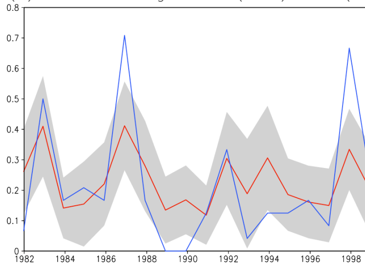
(b) Pacific Trough NCEP(blue), GCM(red)
