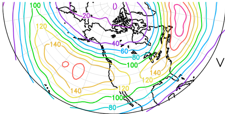
NCEP BP V-var CLIM
