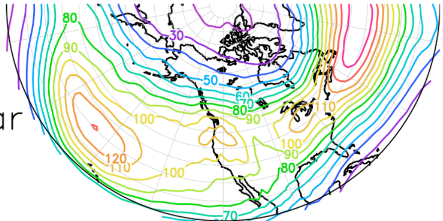
CCSM3 BP V-var CLIM
