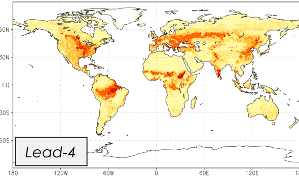
May NMME Total RZ-SM RMSE: Sep (lead-4)
