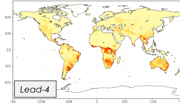
Nov NMME Total RZ-SM RMSE: Mar (lead-4)
