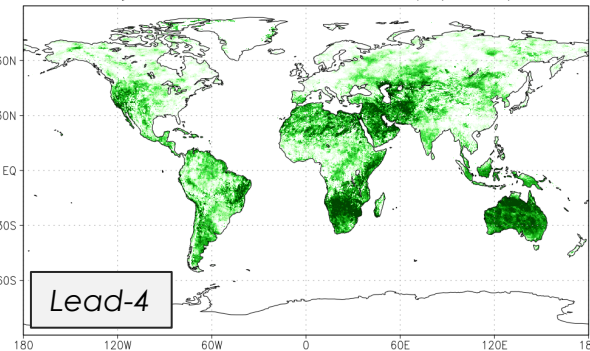
May NMME Total RZ-SM Correl: Sep (lead-4)
