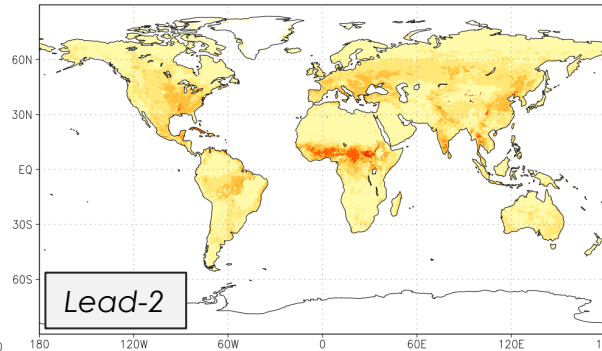
May NMME Total RZ-SM RMSE: Jul (lead-2)
