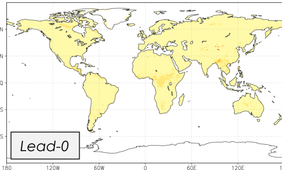
May NMME Total RZ-SM RMSE: May (lead-0)
