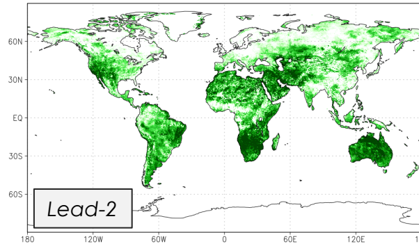
May NMME Total RZ-SM Correl: Jul (lead-2)
