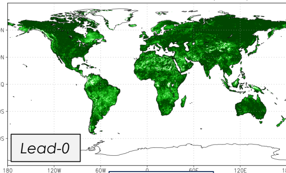
Nov NMME Total RZ-SM Correl: Nov (lead-0)
