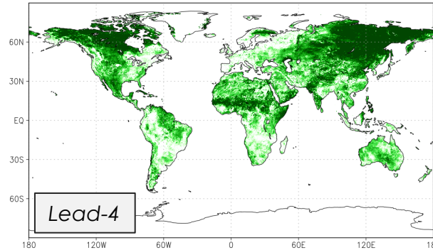
Nov NMME Total RZ-SM Correl: Mar (lead-4)
