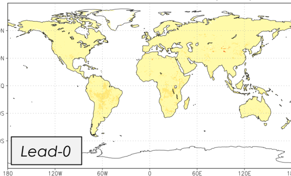
Nov NMME Total RZ-SM RMSE: Nov (lead-0)
