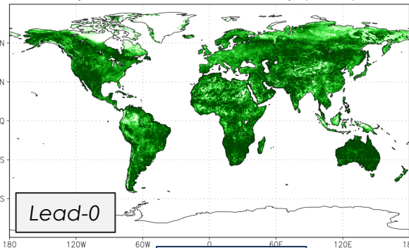
May NMME Total RZ-SM Correl: May (lead-0)
