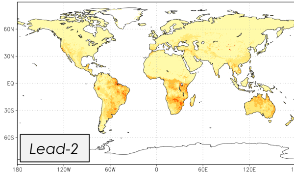
Nov NMME Total RZ-SM RMSE: Jan (lead-2)
