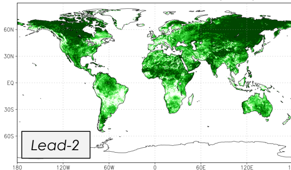
Nov NMME Total RZ-SM Correl: Jan (lead-2)
