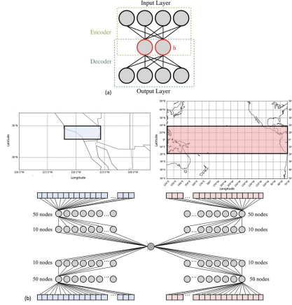
Figure 1. A simple autoencoder architecture (a), MIMO-AE architecture for two inputs and their reconstructions: tropical Pacific SST anomalies and Southern California precipitation anomalies (b). Figure reproduced from Passarella and Mahajan (2023).
