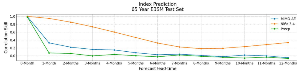
Figure 6. Correlation skill between LSTM-predicted values and true values of MIMO-AE index (blue), Niño 3.4 index (orange), and domain averaged SC-PRECIP at forecast lead times of 0 to 12 months for E3SM testing data.
