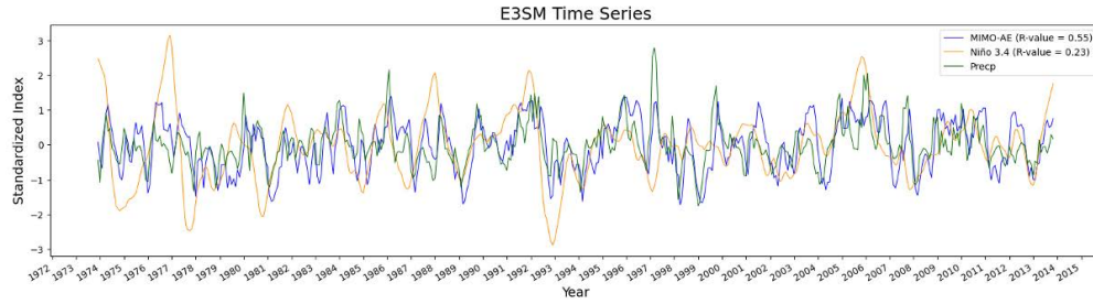
Figure 5. Three-month moving average of the standardized time series of MIMO-AE index (blue), Niño 3.4 index (orange), and domain average SC-PRECIP (green) for a segment (last 40 years: 1974-2013) of the 65 years of E3SM historical simulation testing data.
