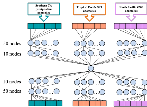
Figure 2. Three input-output MIMO-AE architecture consisting of tropical Pacific SST, Southern California precipitation, and additional North Pacific Z500 anomaly input-output.
