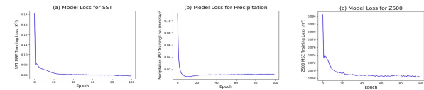
Figure 3. Training Losses for MIMO-AE over 100 epochs using scaled data for tropical Pacific SST (a); Southern California precipitation (b); and North Pacific Z500 anomalies (c).
