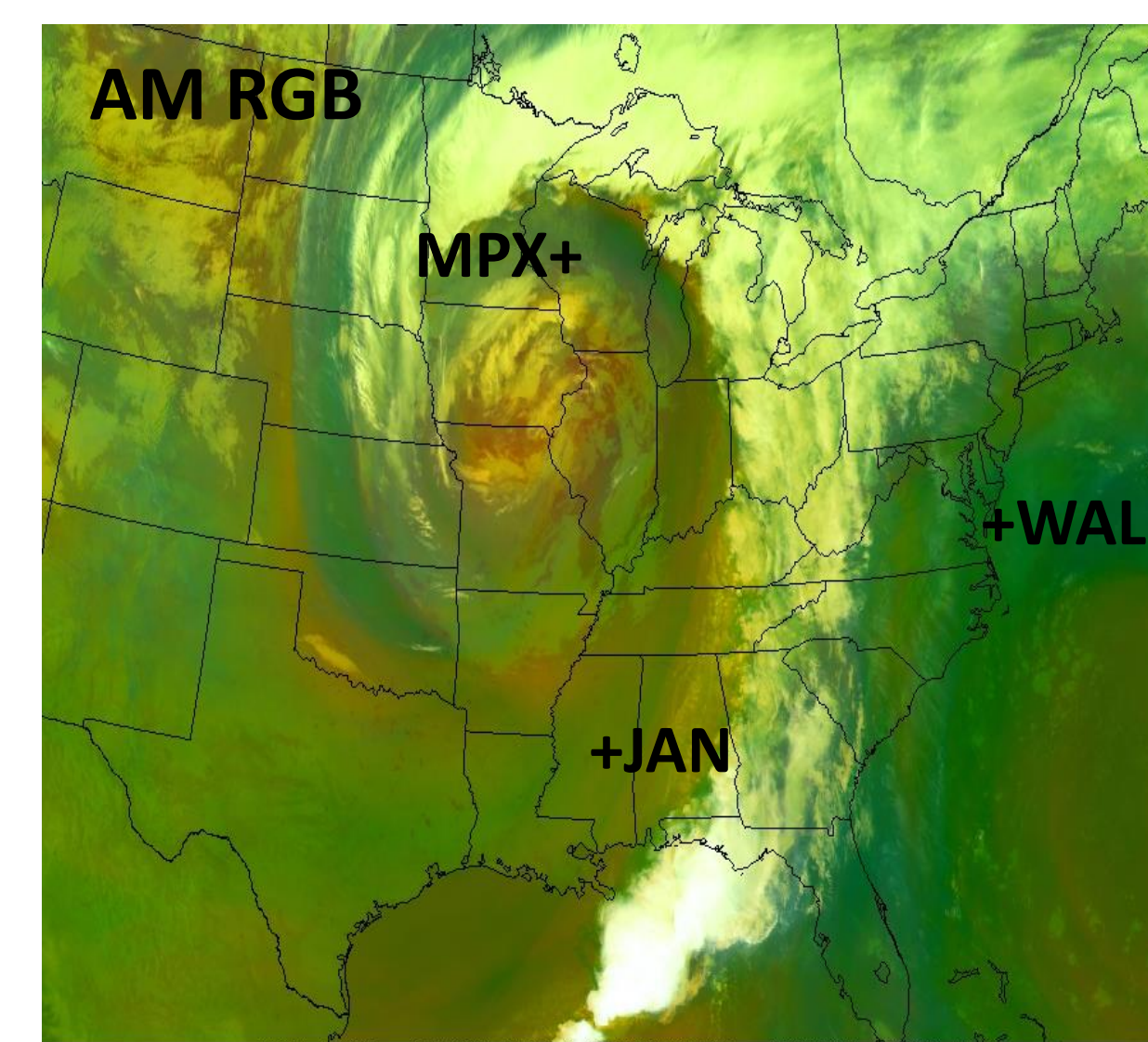
Fig. 9 Limb Corrected Air Mass RGB 1200 UTC 01 May 2018
