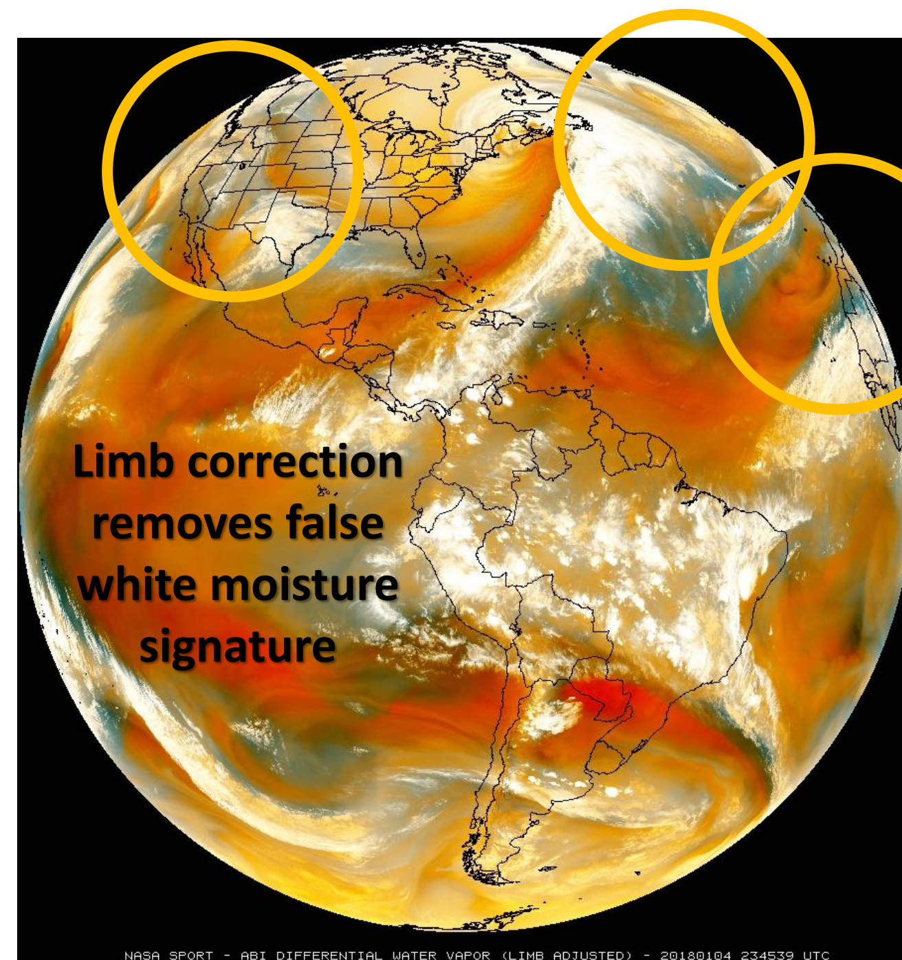
Fig. 4 Limb Corrected Differential Water Vapor RGB 2345 UTC 04 January 2018
