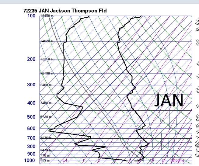
Fig. 11 Jackson, MS sounding 1200 UTC 01 May 2018
