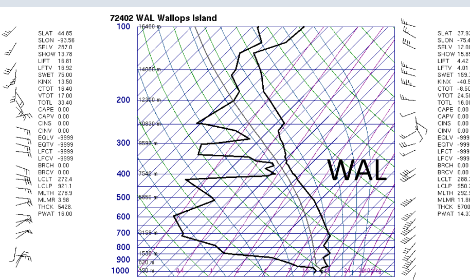
Fig. 13 Wallops Is., VA sounding 1200 UTC 01 May 2018
