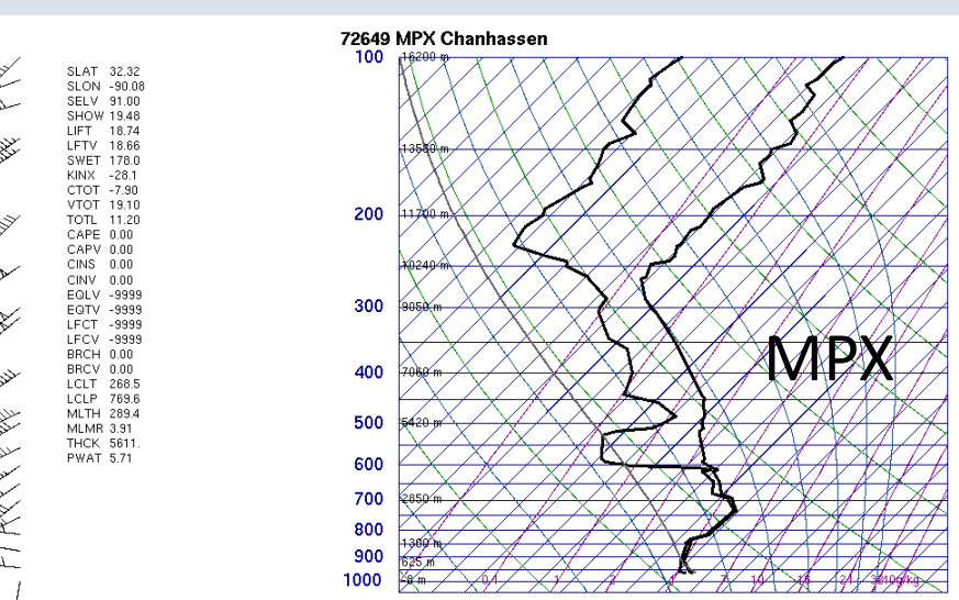
Fig. 12 Chanhassen, MN sounding 1200 UTC 01 May 2018
