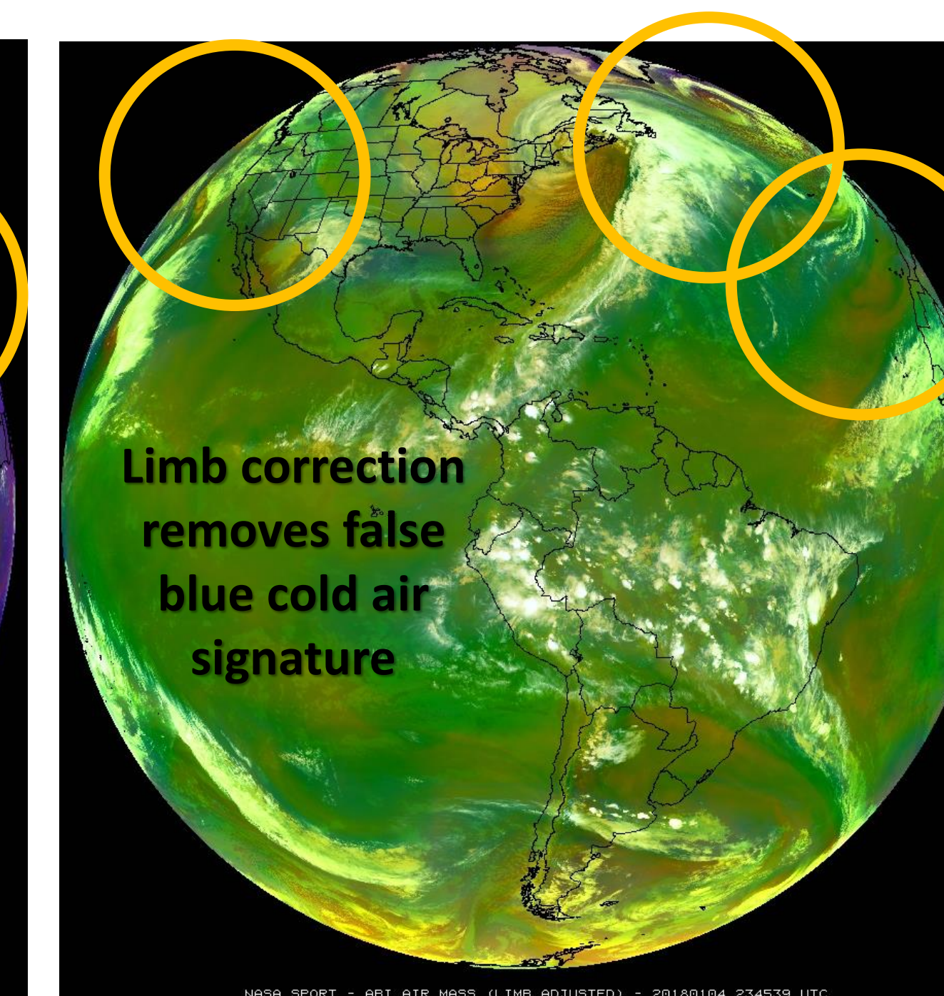
Fig. 2 Limb Corrected Air Mass RGB 2345 UTC 04 January 2018
