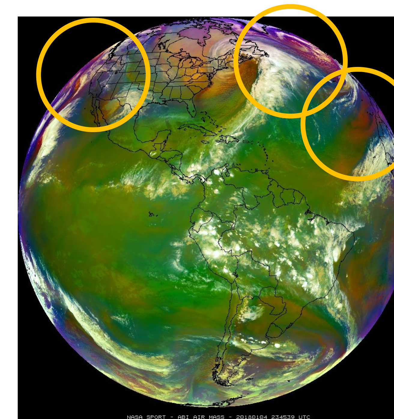
Fig. 1 Air Mass RGB 2345 UTC 04 January 2018
