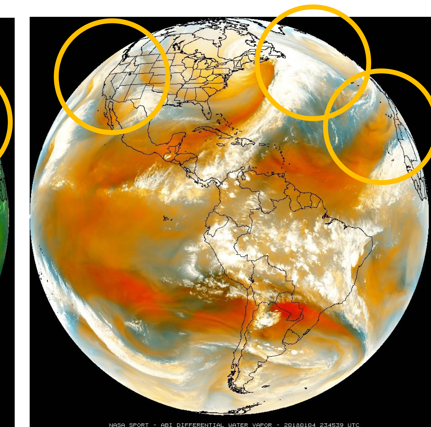
Fig. 3 Differential Water Vapor RGB 2345 UTC 04 January 2018
