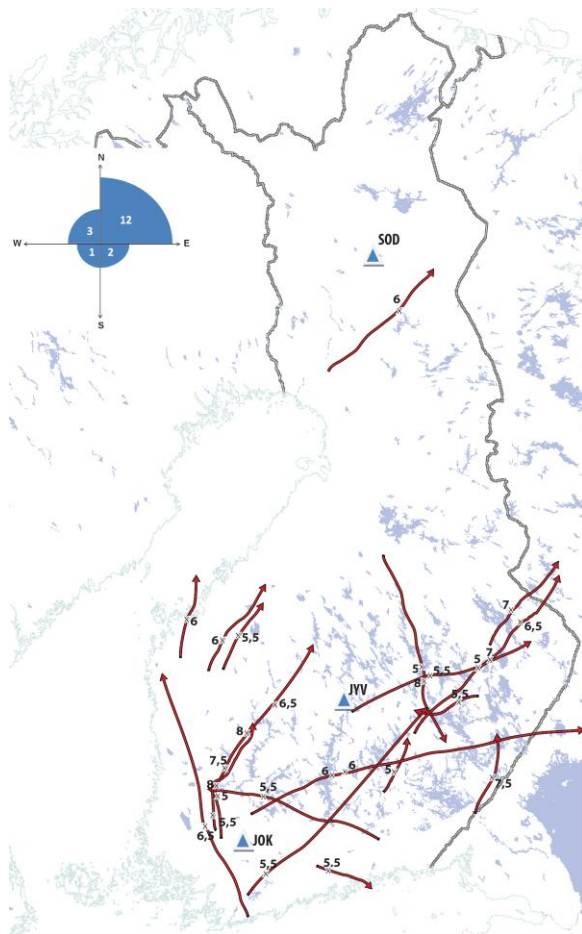
Fig. 2. All significant-hail observations 1999–2011 with hail diameter (cm) and their parent storm tracks. JOK (Jokioinen), JYV (Jyväskylä) and SOD (Sodankylä) indicate sounding stations.
