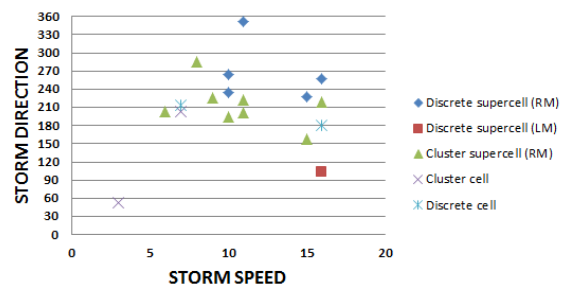
Fig. 4. Parent storm direction of movement (degrees) and speed of motion (m/s).
