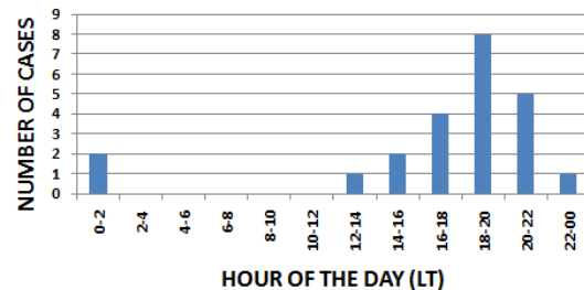
Fig. 1. Diurnal distribution of significant-hail observations 1999–2011 in 2-h periods.
