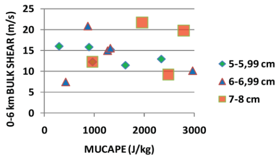
Fig. 3. MUCAPE (J/kg) and 0–6 km bulk shear (m/s) for all 14 known significant-hail days in Finland 1999–2011.
