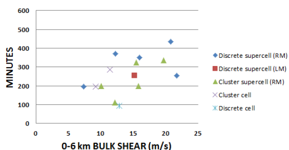
Fig. 6. Parent storm lifetime (minutes) and 0–6 km bulk shear (m/s).
