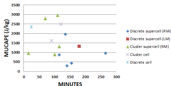
Fig. 5. MUCAPE (J/kg) and time from storm onset to the first significant-hail report (minutes).
