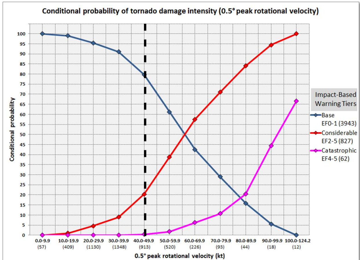
Figure 10. As in Fig. 3, but annotated (black dashed line) on the 40.0-49.9 kt bin for the Case 1 0.5° peak rotational velocity (49 kt).
