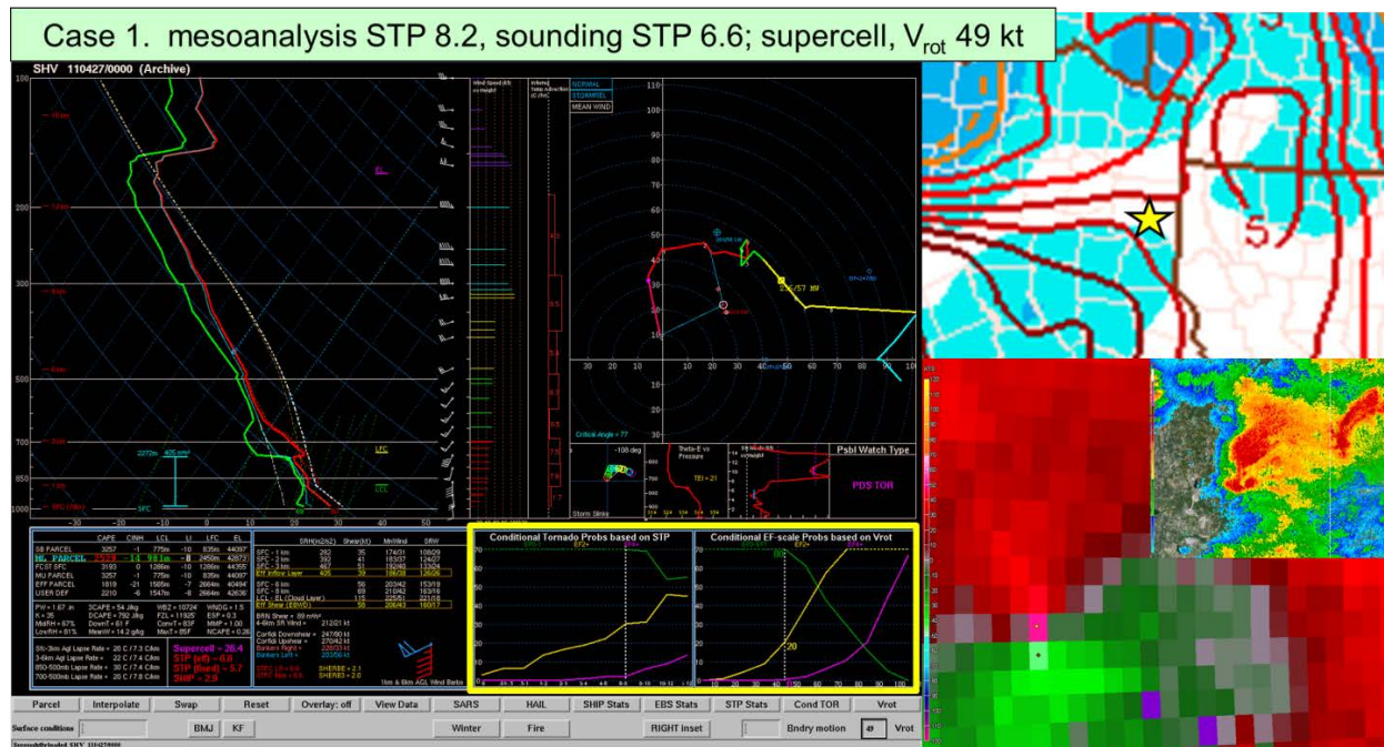
Figure 8. Case 1 (labeled top) with mesoanalysis STP 185km (8.2), sounding STP (6.6), supercell convective mode, and 0.5° peak rotational velocity [ (V_{rot}) 49 kt]. Lower left, an observed proximity sounding display with annotated yellow rectangle highlighting conditional tornado probabilities for STP and 0.5° peak rotational velocity. Lower right . 0.5° storm rotational velocity and middle right (0.5° base reflectivity). Top right mesoanalysis STP with annotated yellow star depicting event location.
