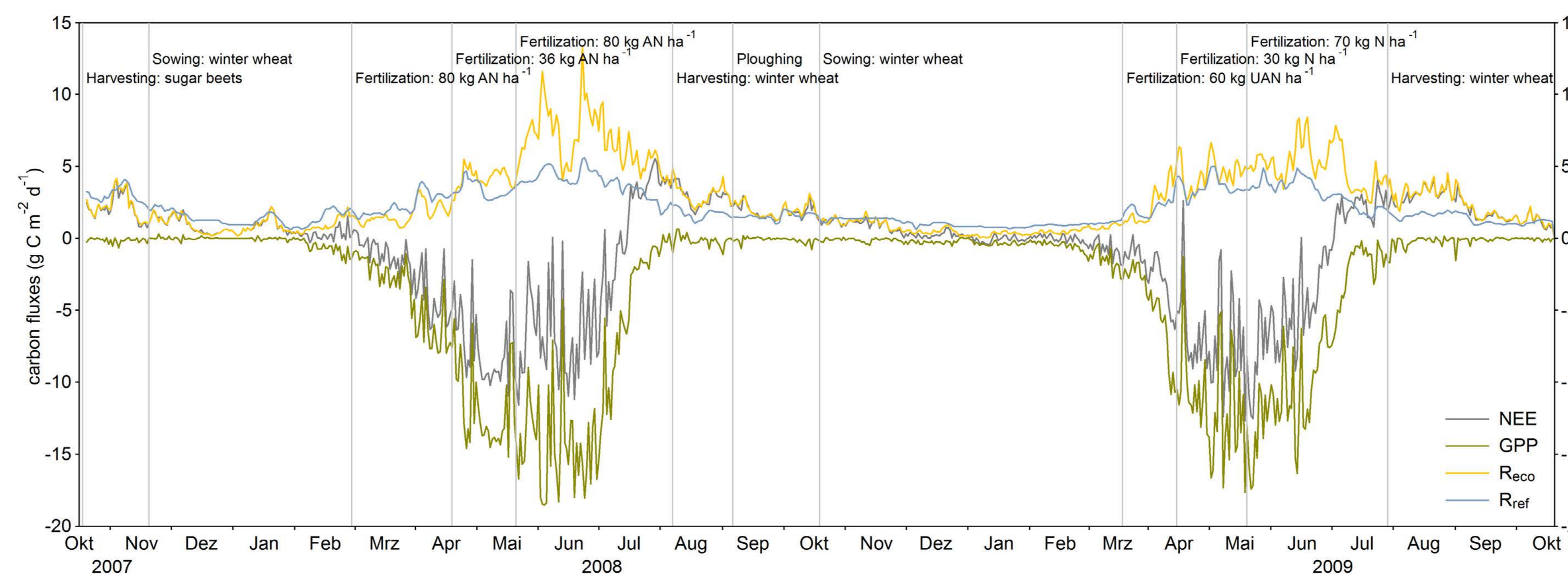
Fig. 3: Daily integrated net ecosystem exchange (NEE), gross primary productivity (GPP), ecosystem respiration ( R_{eco} ) and ecosystem respiration at a reference temperature of 10^\circ\text{C} ( R_{ref} ). Vertical lines indicate important management activities.
