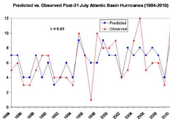
Figure 1: Real-time forecasts of post-31 July hurricanes issued by the TMP from 1984-2010.
