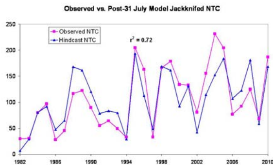
Figure 3: Observed versus post-31 July model jackknifed NTC hindcast over the period from 1982-2010. The three-predictor model explains 72 percent of the variance in post-31 July NTC.
