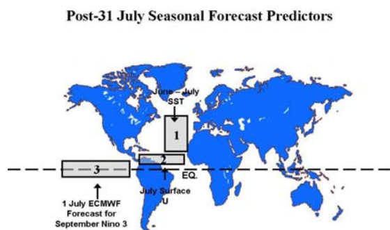
Figure 2: Predictors selected for the new early August statistical forecast model for post-31 July NTC in the Atlantic basin.
