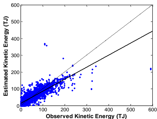
Figure 2: Scatter plot of observed total IKE values vs. estimated total IKE values from a 24-hour SPIKE regression model (blue dots). The dark black line represents the best fit line between the 4239 observed and estimated data points. The dashed line represents a perfect forecast ( y=x ).
