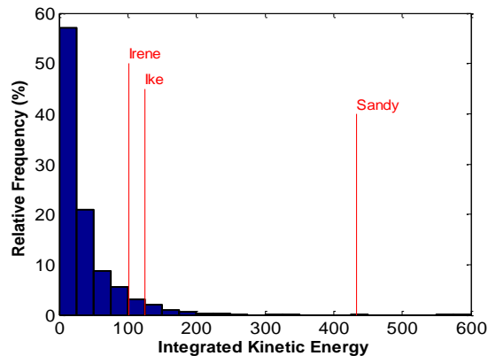
Figure 1: Relative frequency distribution of six-hourly IKE measurements in Atlantic TCs between 1990 and 2011. This sample includes 5498 fixes from 291 storms. Red vertical lines are shown to indicate IKE values for selected hurricanes just prior to a US landfall. The times of these IKE measurements are as follows: Irene 8/26/11 06Z; Ike 9/13/08 00Z; Sandy 10/29/12 18Z.
