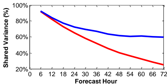
Figure 3: Plot of shared variance over forecast hour for total IKE. The blue line represents the shared variance between the observations and the SPIKE model. The red line represents the shared variance between persistence and the observed IKE value a certain number of hours later.
