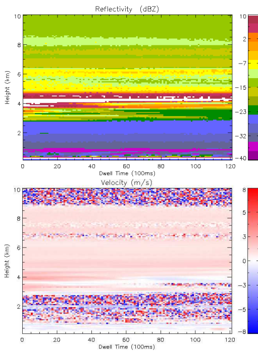
Figure 4: Vertical reflectivity (upper) and velocity (lower) profile at 23:45:07Z , June 1, 2010.
