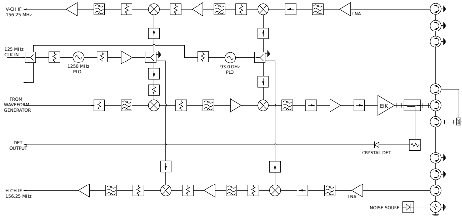
Figure 1: Block diagram of dual-channel polarimetric HCR transceiver.
