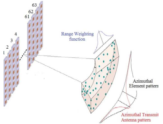
FIG. 2. Conceptual depiction of the phased-array weather radar signal simulator.
