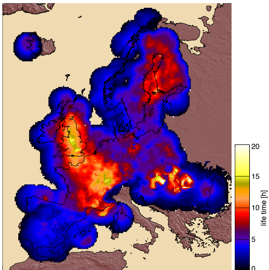
Fig. 5. Average lifetime for the period from 01 June 2012 to 31 May 2013.
