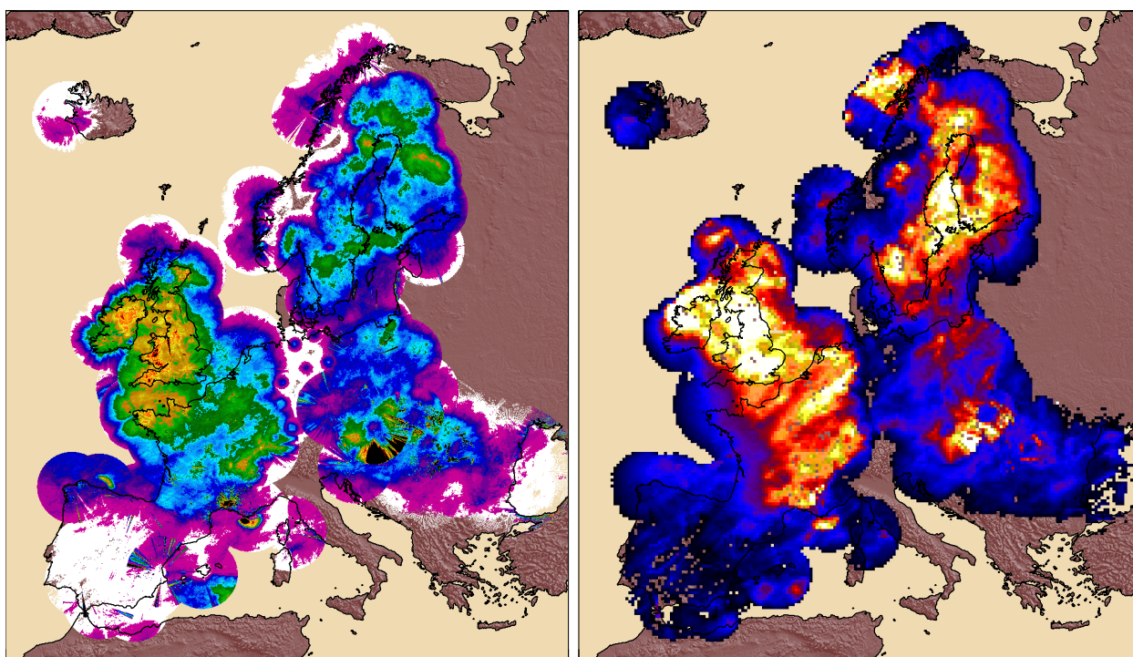
Fig. 6. Frequency of radar echoes exceeding 10 dBZ (left) and average lifetime (right) for the month of June 2012.
