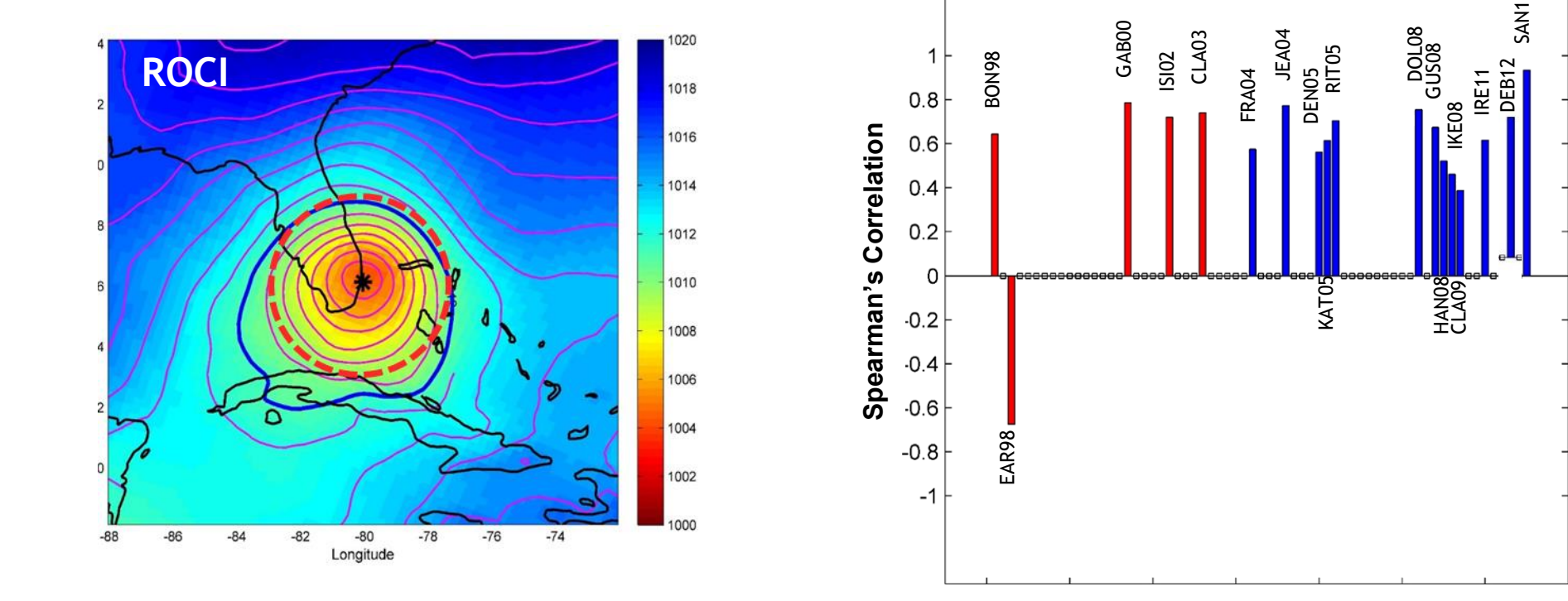
Fig 6. Objectively determined (solid blue) and extended best track (EBT; dashed red) radius of outermost closed isobar (ROCI)
