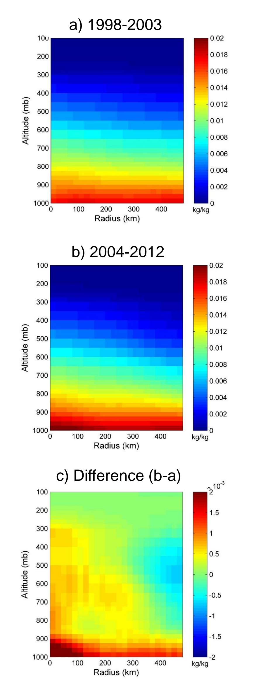
Fig 9. 9-storm Specific Humidity Composites
