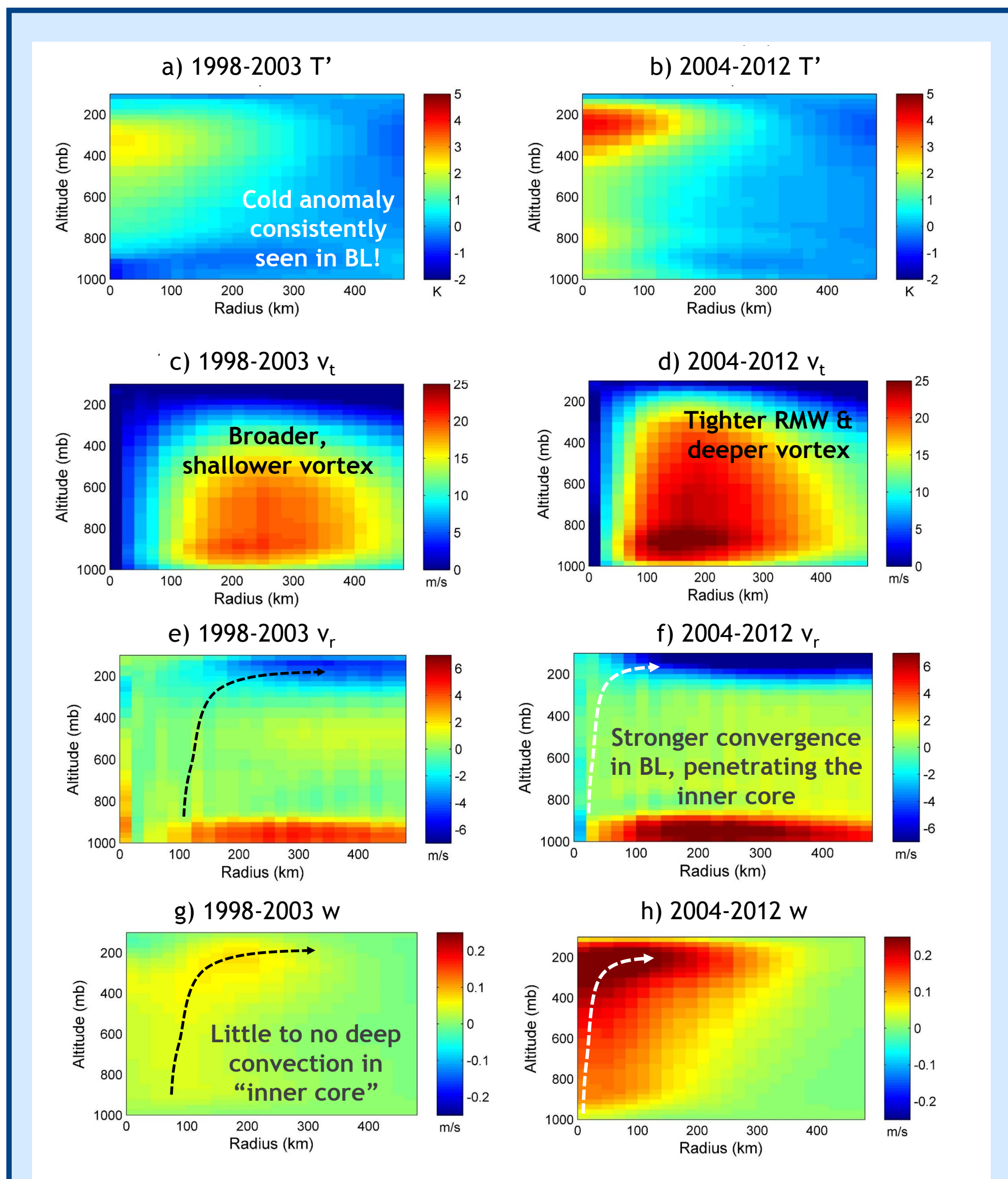
Fig 8. 9-storm composite radial cross section of azimuthally averaged temperature perturbations and winds
