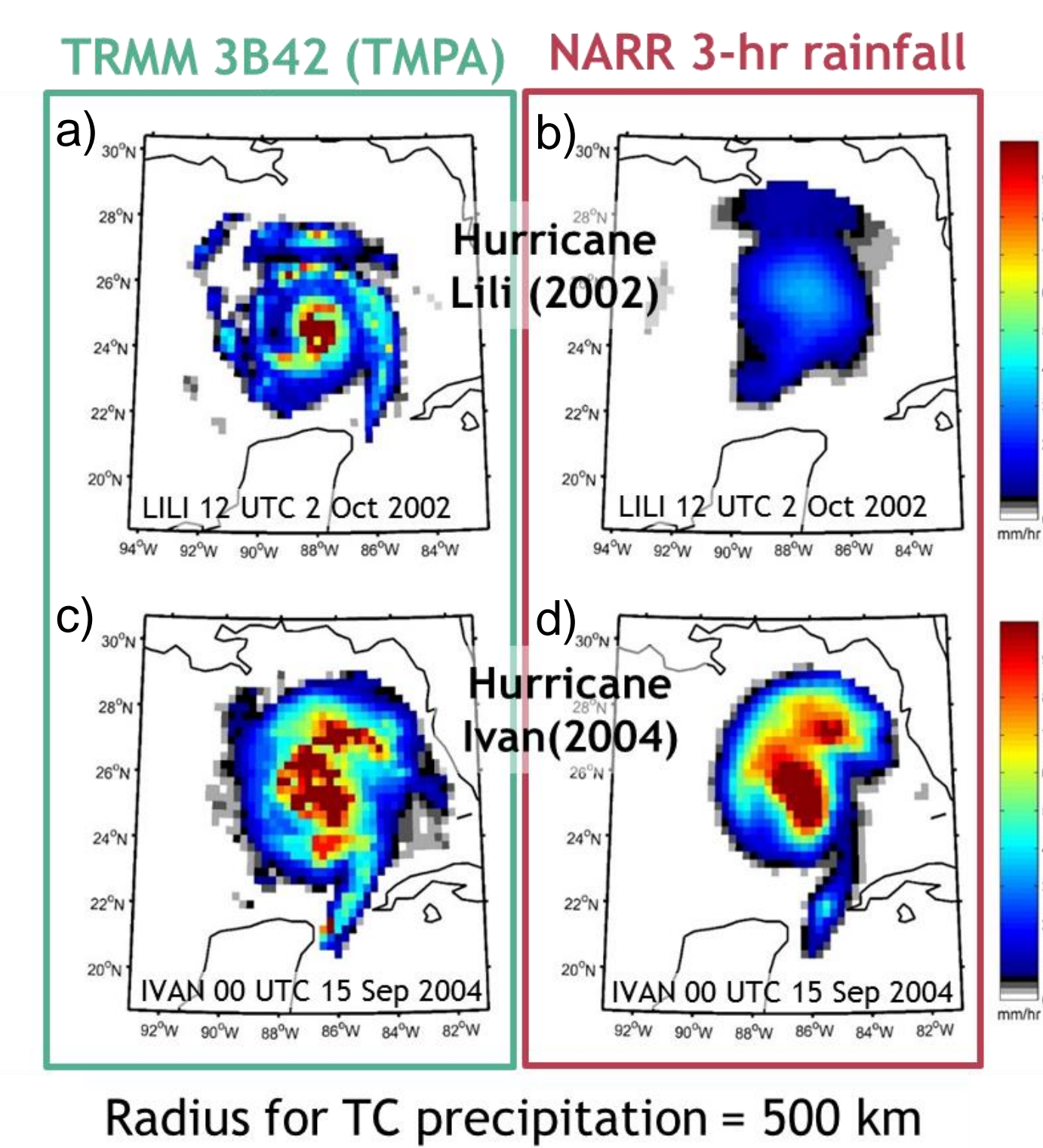
Fig 3. Precipitation structures in (left) TRMM 3B42 and (right) NARR data sets: (a and b) Hurricane Lili (2002) valid at 12:00 UTC, 2 October and (c and d) Hurricane Ivan (2004) valid at 00:00 UTC, 15 September.
