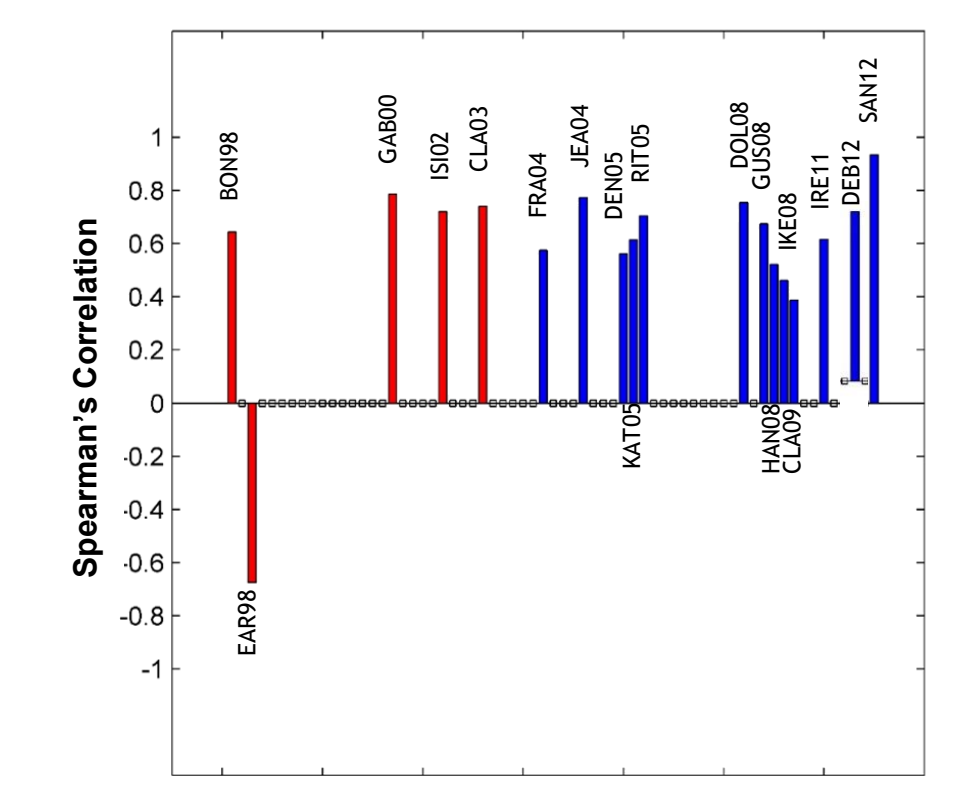
Fig 7. Mean lifetime ROCI in NARR vs EBT and Spearman's correlation coefficients ( p < 0.05 ) for evolution of ROCI
