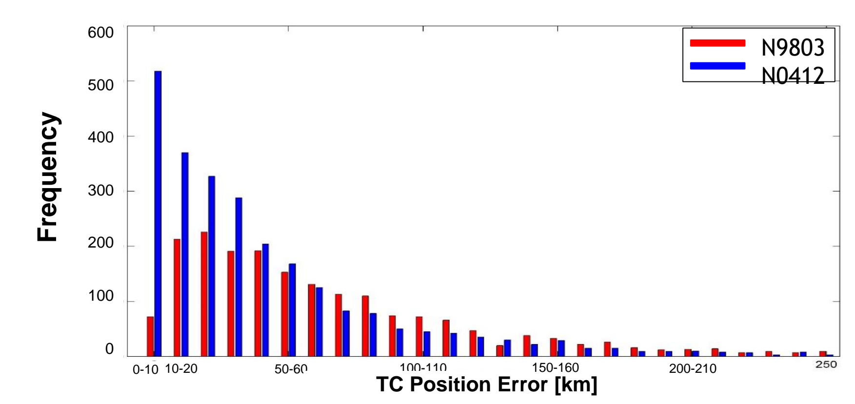
Fig 5. TC position error frequency distributions. Bin widths are 10 km.
