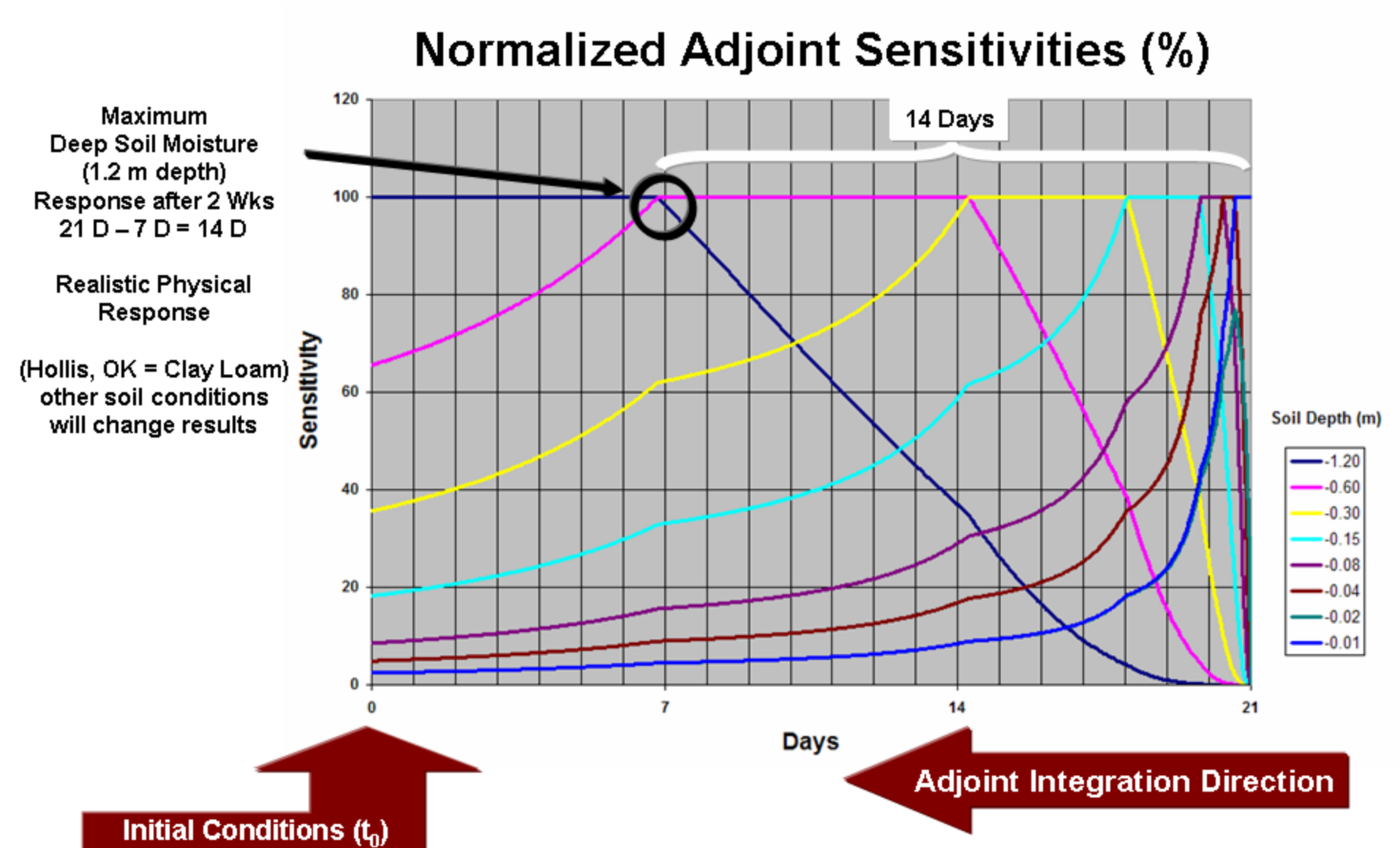
Figure 2: Normalized adjoint sensitivity results for Hollis, OK case study. Deep soil moisture at a depth of approximately 1 m has the largest sensitivity in the integration time period of 0-7 days. This indicates the strong deep soil moisture sensitivity as a function of soil depth with time.
