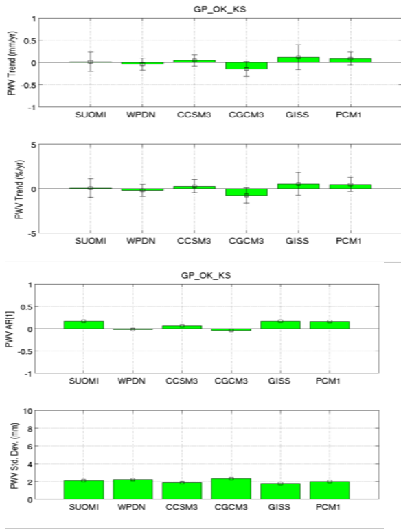
Figure 4. SuomiNet, WPDN, and GCM trends (top panel) and autocorrelation (bottom panel) and standard deviation (bottom panel) for the Oklahoma/Kansas region from 2000-2010.
