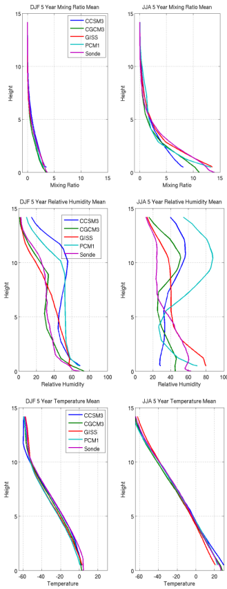
Figure 7. Mean GCM and ARM SGP radiosonde profiles for winter (DJF) and summer (JJA) over the period 2005-2010 for mixing ratio, relative humidity, and temperature.
