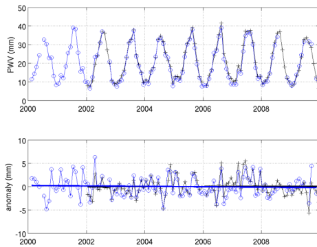
Figure 2. Monthly mean PWV (upper panel) and anomaly time series with trend fits (lower panel) in the Oklahoma/Kansas region for the arithmetic mean of SuomiNet (plus symbol) and NOAA WPDN (circles) GPS stations.
