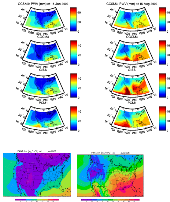
Figure 6. Map plots of GCM PWV compared to the NARR (bottom) for the month of January (left) and August (right) 2006.
