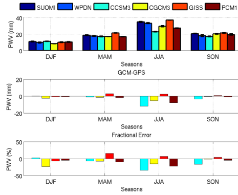
Figure 5. (upper) PWV mean (2000-2010) for the Oklahoma/Kansas region with error bars representing the uncertainty in the mean estimate ( k=1 ). (middle) GCM-GPS PWV difference. (lower) GCM fractional error relative to GPS PWV observations.
