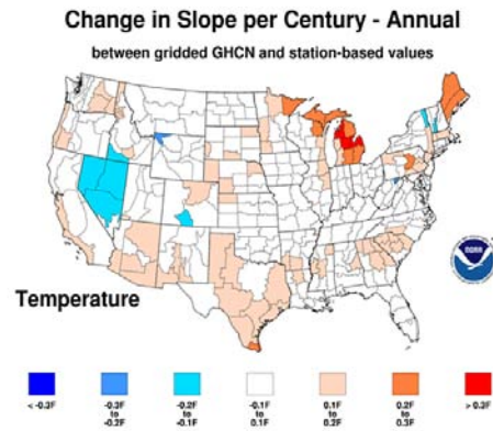
Figure 2. Difference in slope (trend) between the Gridded GHCN-D (GrDD) and Traditional (TCDD) methods of calculating (a) precipitation (inches per century) and (b) temperature (degrees Fahrenheit per century). Compared to the TCDD, the GrDD has a more positive precipitation trend in Maine, drier in Alabama, warmer in Michigan, and cooler in Nevada. These reflect peculiarities related to the regression methods used to obtain the averages prior to 1930 (see text for details).
