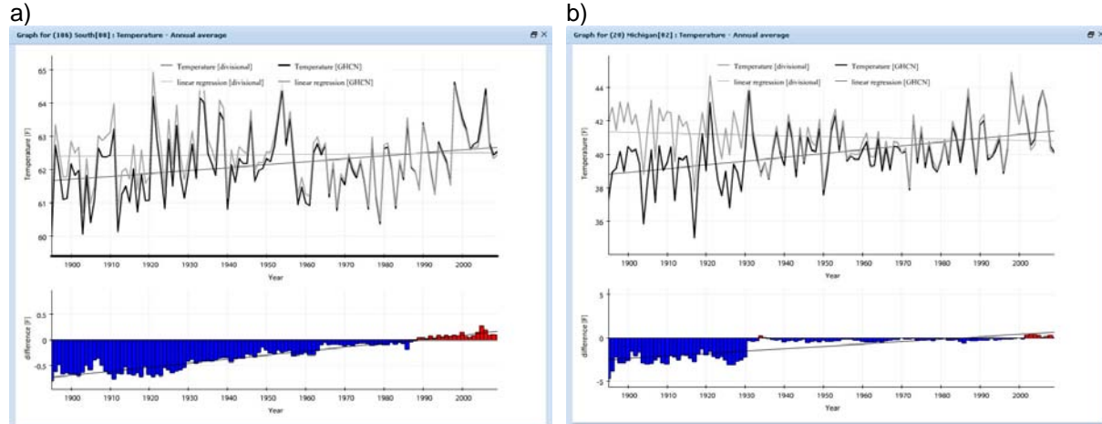
Figure 3. Average annual temperature comparison for (a) the South climate region (a composite of Arkansas, Kansas, Louisiana, Mississippi, Oklahoma, and Texas) and (b) Michigan Climate Division 2. The bottom panel in each shows the difference (GrDD minus TCDD) between the two data sets. Please note that the scales for each panel are very different. During the past 20-years, the GrDD is warmer than the TCDD (red bars). For Michigan CD2, the impact of eliminating the pre-1930s regression methods can be clearly seen. The tool used to construct these comparisons is publicly available at: http://
