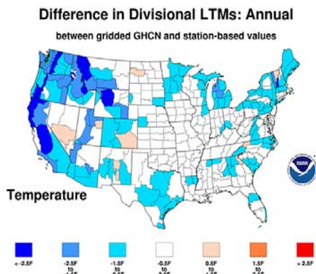
Figure 1. Difference in long-term means (LTMs) between the Gridded GHCN-D (GrDD) and Traditional (TCDD) methods of determining climate division (a) precipitation (inches), and (b) temperature (degrees Fahrenheit). Mountainous climate divisions in the West tend to show cooler and wetter LTMs in the GrDD method. GHCN-D closely follows the traditional divisional dataset east of the Rockies.
