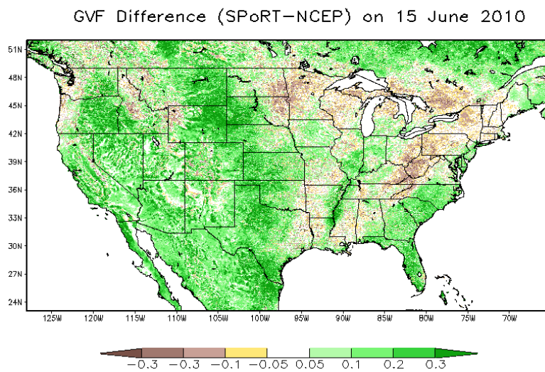
Figure 2. Depiction of the greenness vegetation fraction (GVF) on the SPoRT CONUS 0.01° domain from 15 June for the current NCEP/AVHRR climatology (top), the SPoRT daily GVF (middle), and the difference (SPoRT – NCEP, bottom).
