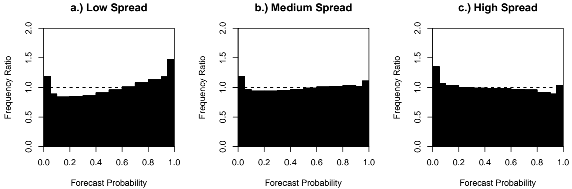
Fig. 8: PIT histograms for 102-h 2-m temperature. Forecasts have been stratified into low (a), medium (b), and high (c) spread cases using station-specific thresholds. The PITs were created using the full set of 2303 stations.
