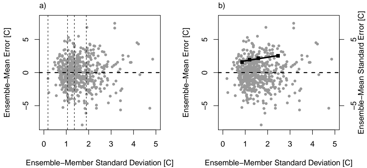
Fig. 1: Scatter plots illustrating spread-skill relationship development. The ensemble-member standard deviation is plotted along the abscissa while the error of the ensemble-mean is plotted along the ordinate. Each dot represents one forecast case. The vertical dashed lines (Fig. 1a) are the breakpoints used to bin cases. In Figure 1b the black squares are the bin-calculated values for the ensemble-mean standard error while the black line is the spread-skill relationship.
