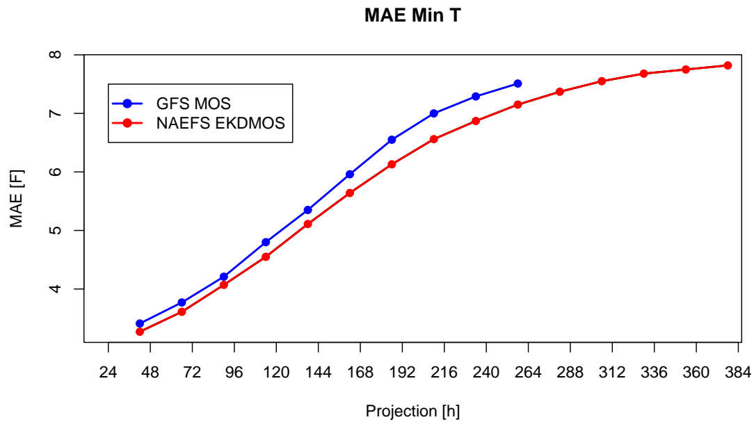
Fig. 5: Same as Figure 2 but for nighttime minimum temperature.
