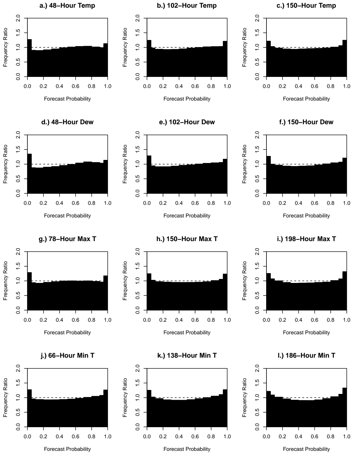
Fig. 6: PIT histograms for 2-m temperature (a-c), dewpoint (d-f), daytime maximum temperature (g-i) and nighttime minimum temperature (j-l).
