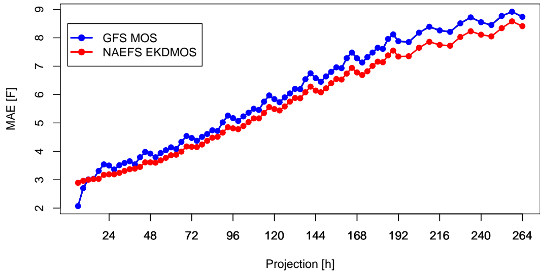
Fig. 3: Same as Figure 2 but for dewpoint.
