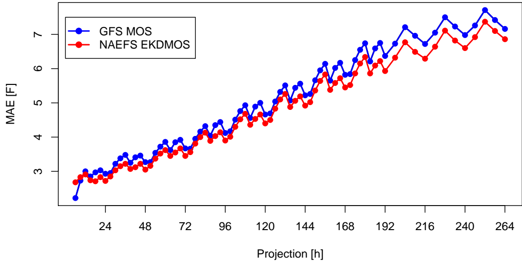
Fig. 2: Cool season 2-m temperature MAE plotted by projection.
