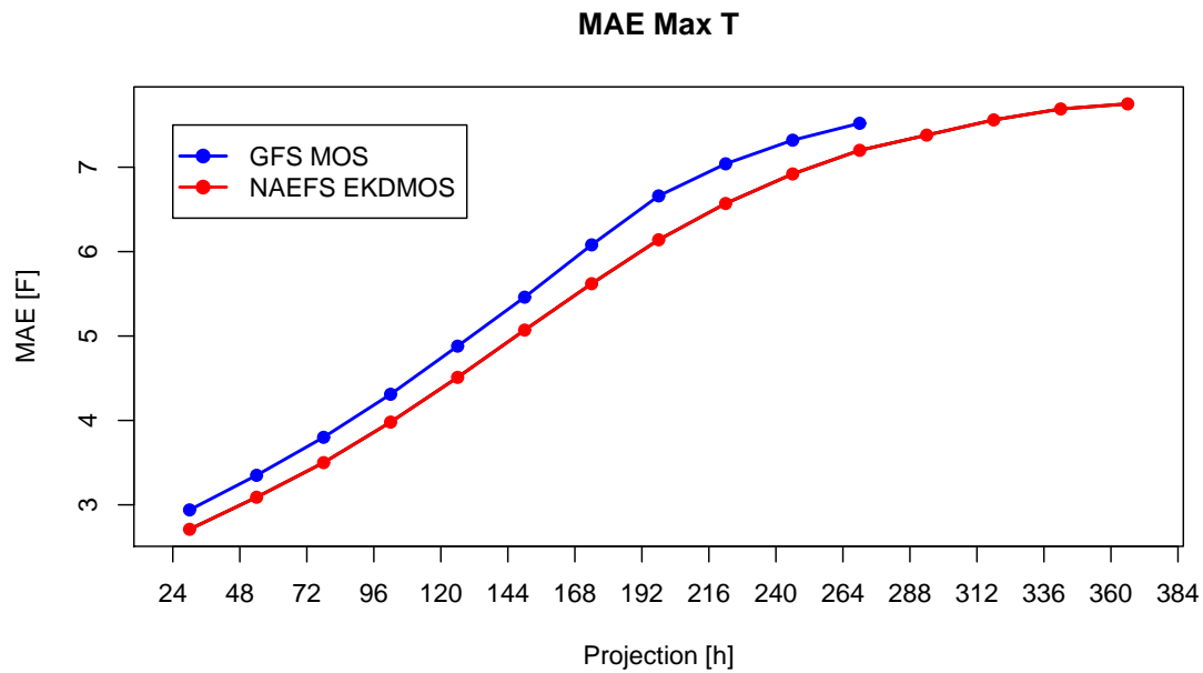
Fig. 4.: Same as Figure 2 but for daytime maximum temperature.
