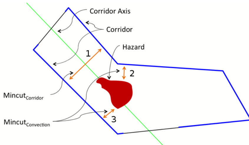
Figure 1. Conceptual model of the Flow Constraint Index. Blue lines represent the corridor boundaries. The red area denotes an area of hazardous weather. Arrow 1 represents the distance across the corridor in the absence of hazards. Arrows 2 and 3 show the distance across the available airspace around a hazard. The flow constraint is a function of the ratio of these two distances.
