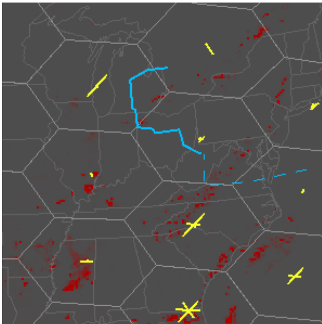
Figure 4. CIWS VIL 3.5 field (red), FCI (yellow lines, length of line represents extent of constraint), A05 (solid blue line) and A08 (dashed blue line) for 1900 UTC 18 August 2011.
