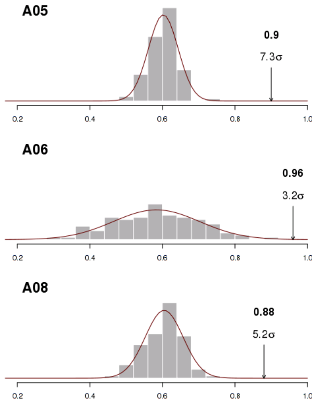
Figure 5. Histograms (gray bars) and fitted normal distribution (red line) for the CSI of the random pairings of FCI fields and AFP states. Bold numbers denote the skill of the classification model for the true pairings. Light numbers denote the number of standard deviations between the true model skill and the mean of the corresponding distribution.
