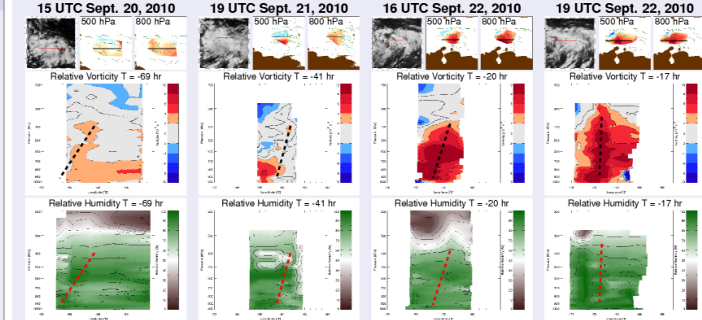
Fig. 3. As in Fig. 2, except for the developing Pre-Matthew system which was declared a tropical depression on Sept. 23 at 12 UTC.
