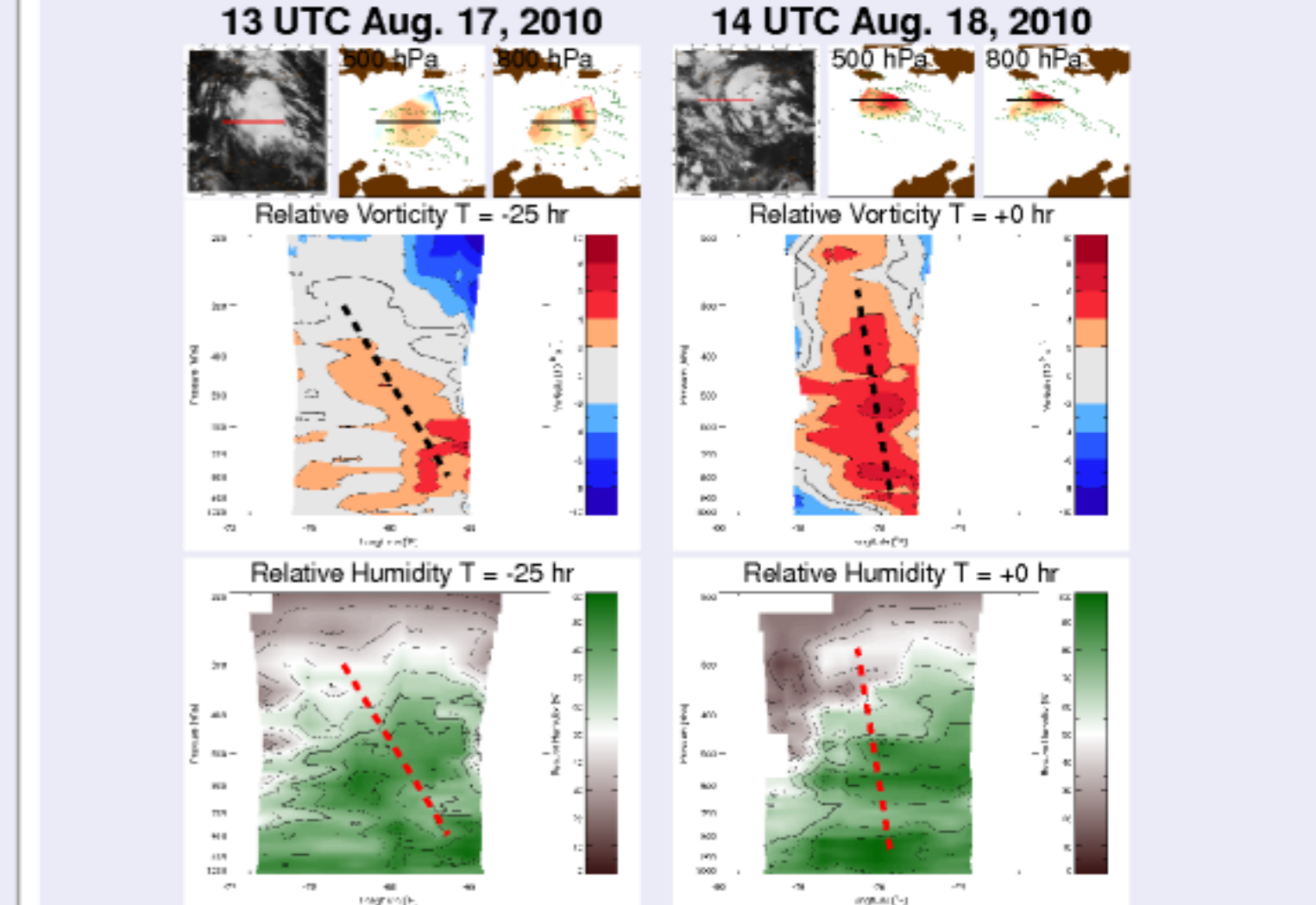
Fig. 4. As in Fig. 2, except for the non-developing PGI27L system.
