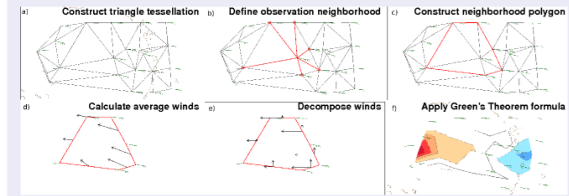
Fig. 1. Visual outline of method for calculating vorticity using Green's Theorem on polygonal regions (from Helms and Hart 2012).
