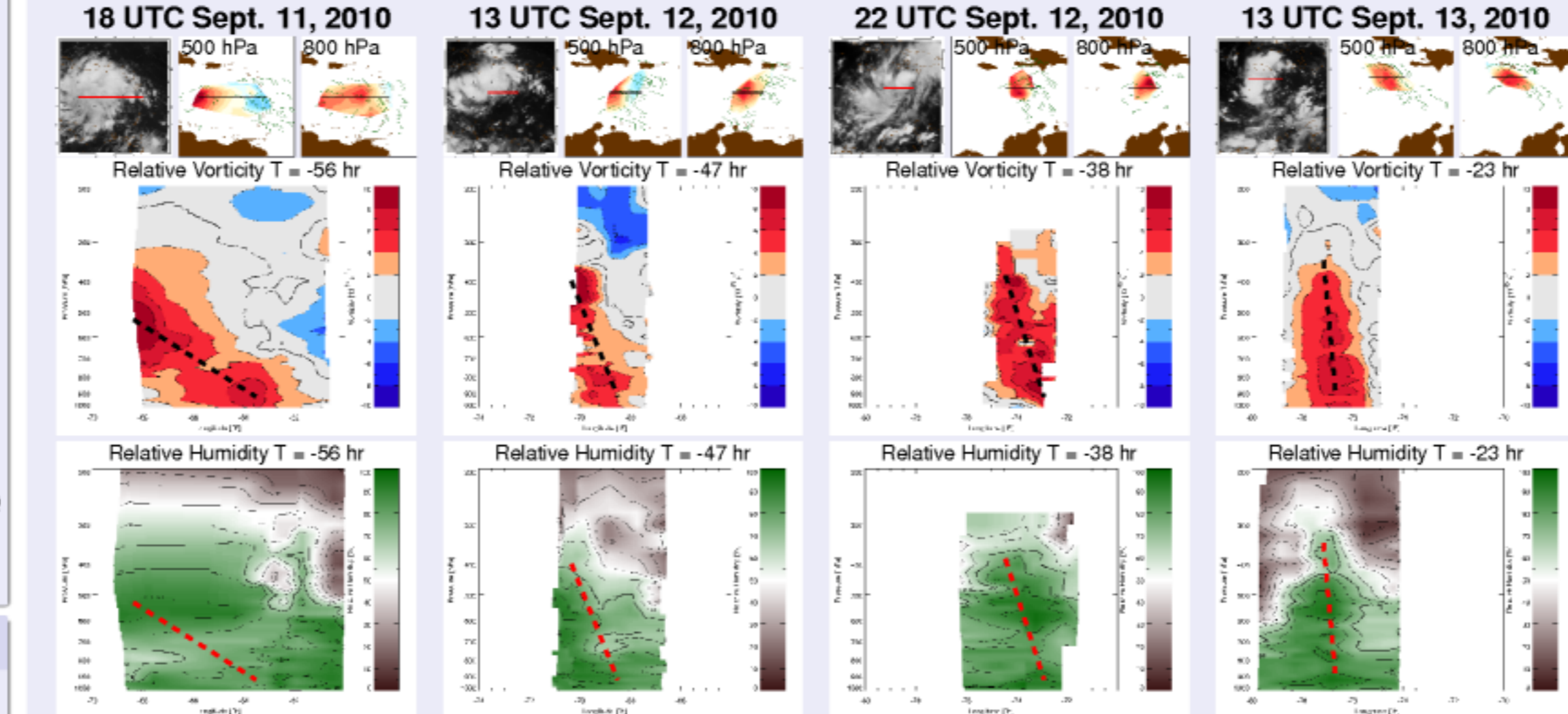
Fig. 2. Series of cross-sections (earlier times on left) from the developing Pre-Karl system which was declared a tropical depression on Sept. 14 at 12 UTC. For each time, plots of the corresponding IR satellite image (top row, left), 500 hPa relative vorticity (top row, middle), 800 hPa relative vorticity (top row, right), relative vorticity cross-section (middle row), and relative humidity cross-section (bottom row) are included. The red or black horizontal bars in the satellite image and the 800 hPa and 500 hPa relative vorticity plots represent the location of the cross-section data at the corresponding time. The dashed line in the vorticity and relative humidity cross-sections indicates the approximate axis of maximum vorticity.
