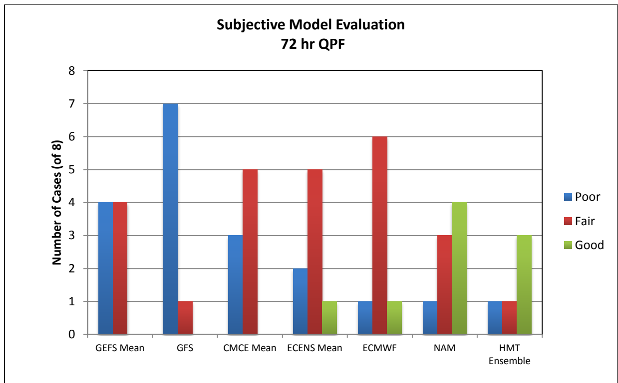
Figure 6) Subjective model performance of the 72 h QPF for each of the guidance systems used in ARRFEX.
