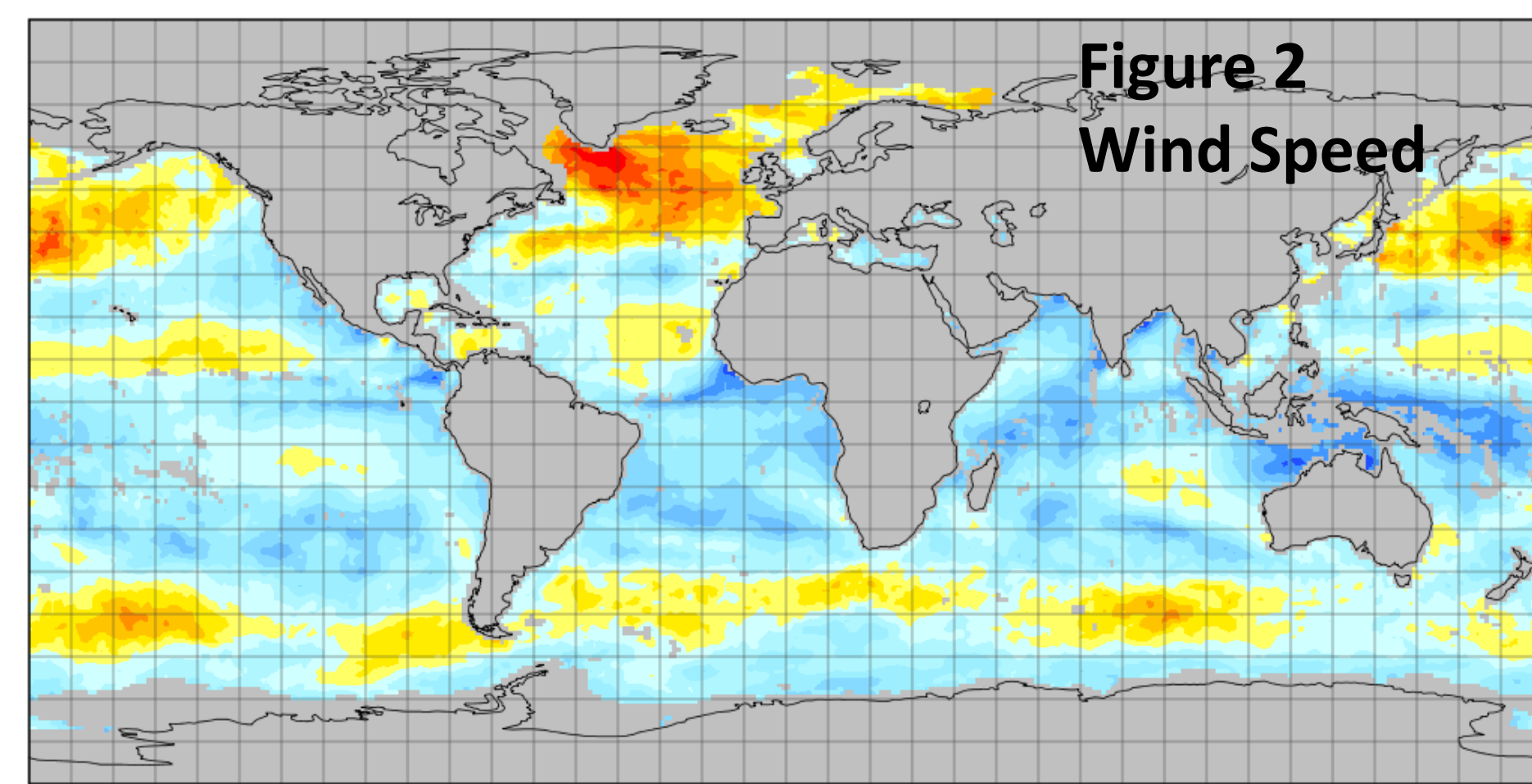
Monthly Average 10m Wind Speed Over Ice-Free Oceans
