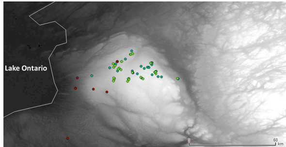
Figure 10. The dark green dots denote the location of detected ENTLN flashes during IOP 7. The lighter green dots denote the location of detected USPLN strokes. The red dots denote human reports of lightning and/or thunder by several mobile snow teams. The lightning data are overlaid onto topographical data, with whites being the highest elevations and dark grays being the lowest.
