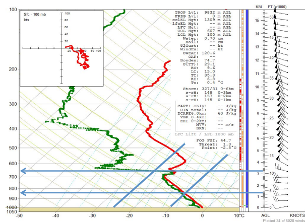
Figure 7. Same as Fig. 6, except for 2007 UTC 18 Dec 2013, Ellisburg, NY and 1.5 hrs before lightning occurrence.
