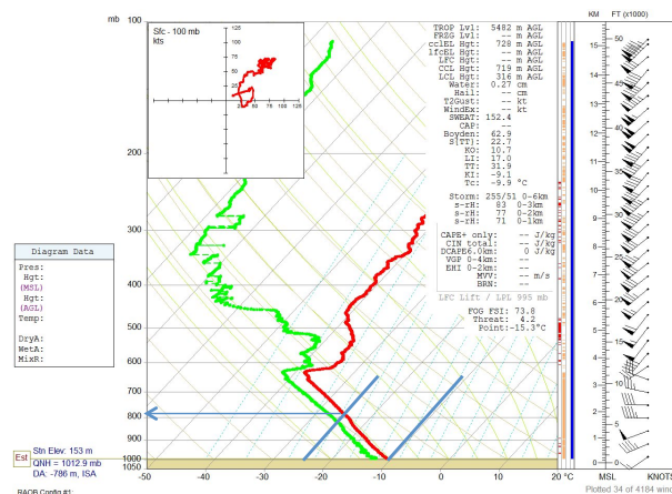
Figure 6. Sounding launched by SUNY Oswego team within lake-effect snow band at Henderson Harbor, NY at 0513 UTC 7 Jan 2014 (1 hr before lightning). The blue lines highlight the area where -25^{\circ}\text{C} \leq T \leq -10^{\circ}\text{C} .
