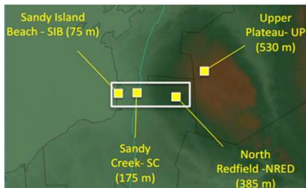
Figure 2. The four MRR transect locations remained stationary throughout the OWLeS Project, starting along the lake shoreline at Sandy Island Beach about 75 m MSL and extending into the highest elevations of the Tug Hill Plateau at 530 m MSL. Courtesy Jim Steenburgh.
