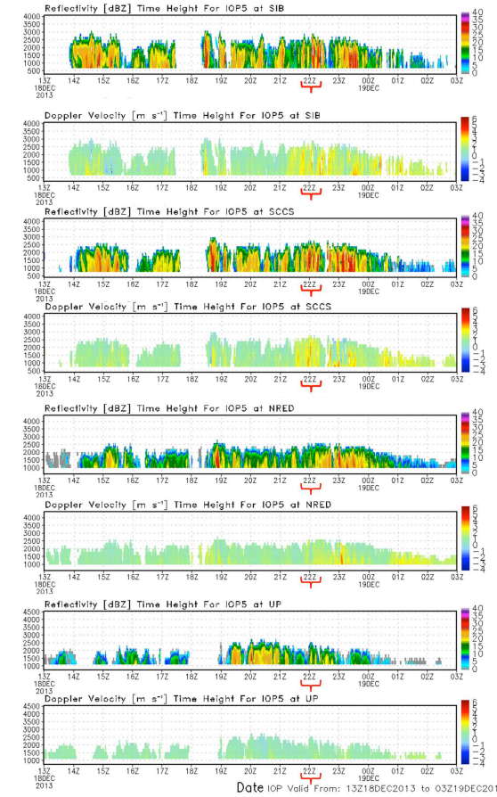
Figure 9. Reflectivity time-height and their corresponding Doppler velocity plots are shown for each of the four MRR transect locations, beginning with the westernmost location at Sandy Island Beach (SIB) and ending with the UP location. The red brackets denote the time period of lightning.
