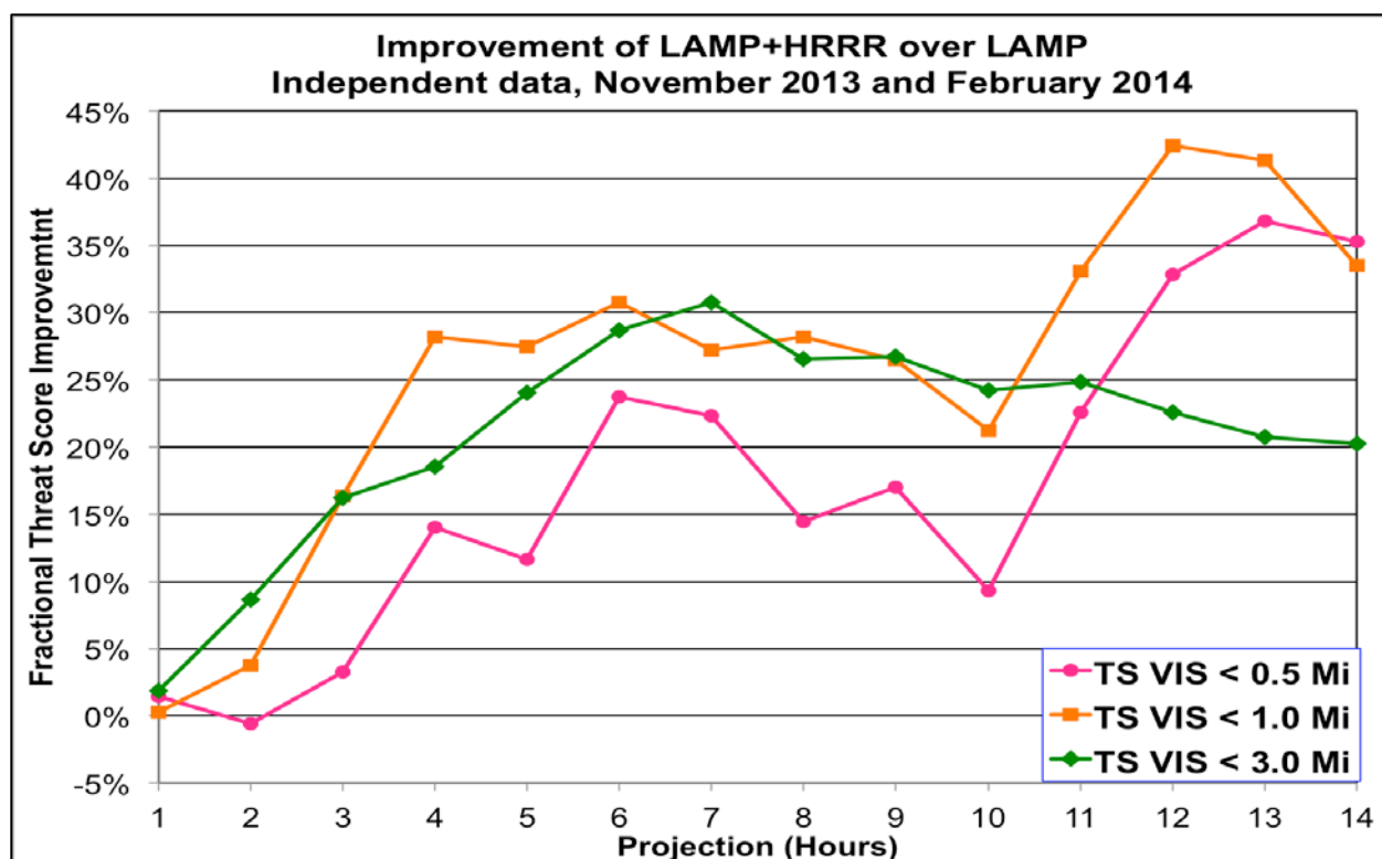
FIG. 5. Improvement in threat score of new 0000 UTC LAMP+HRRR forecasts over threat score of original 0000 UTC LAMP forecasts for visibility < 0.5 miles (pink circles), visibility < 1 mile (orange squares), and visibility < 3.0 miles (green diamonds).
