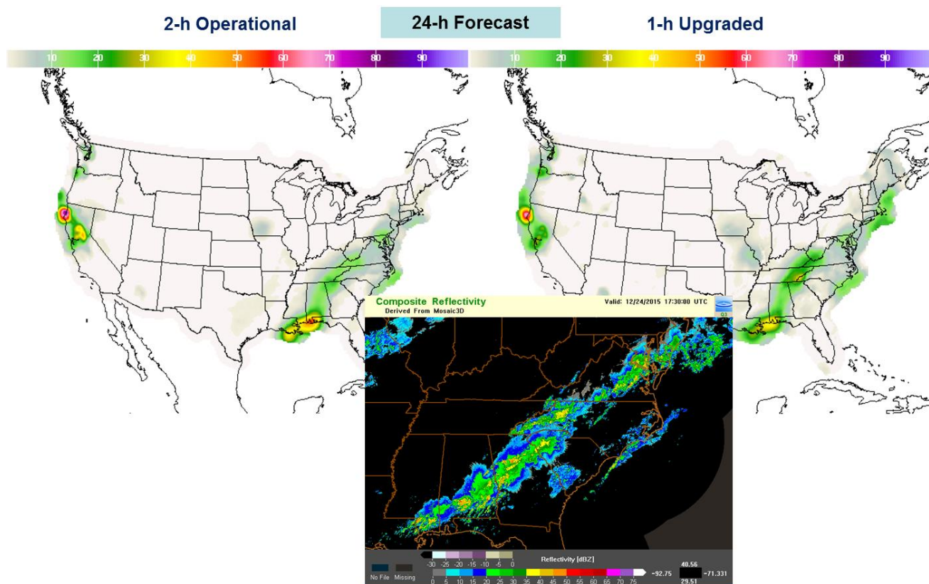
Figure 5c. As in Fig. 5a except for the 24-h forecast projection.
