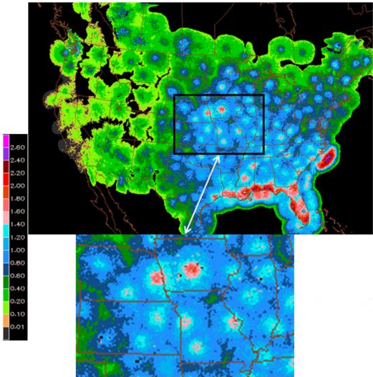
Figure1b. As in Fig. 1a, except after MDL supplemental quality control (QC) processes were applied. Black (missing data) areas inside the MRMS coverage area result from the application of a “static mask” -- a component of the QC processes (see text).
