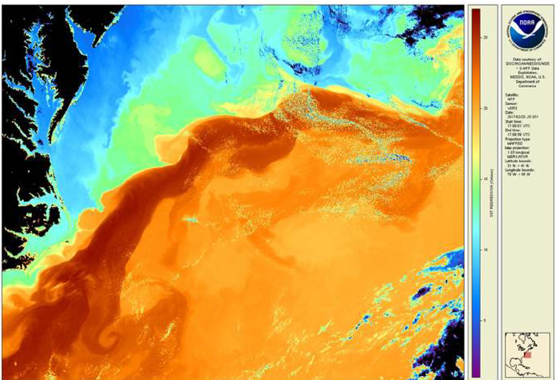
VIIRS Sea Surface Temperature (ACSPO) 2/20/17
