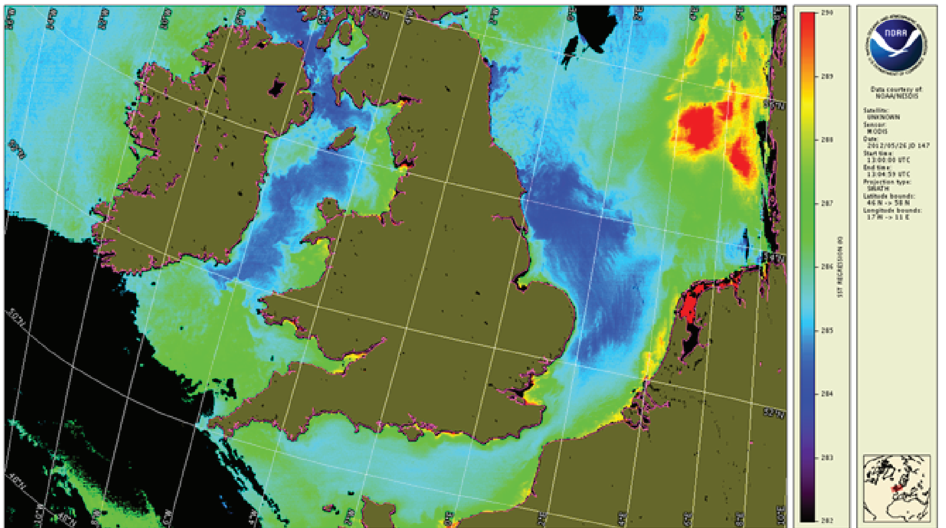
VIIRS Sea Surface Temperature (IDPS) 5/26/12
