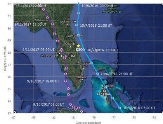
Figure 4. Surface tracks of Hurricanes Irma in 2017 (purple) and Matthew (Blue) in 2016 within proximity to the KSC TDRWP site (yellow star) (Huddleston et al. 2017).
