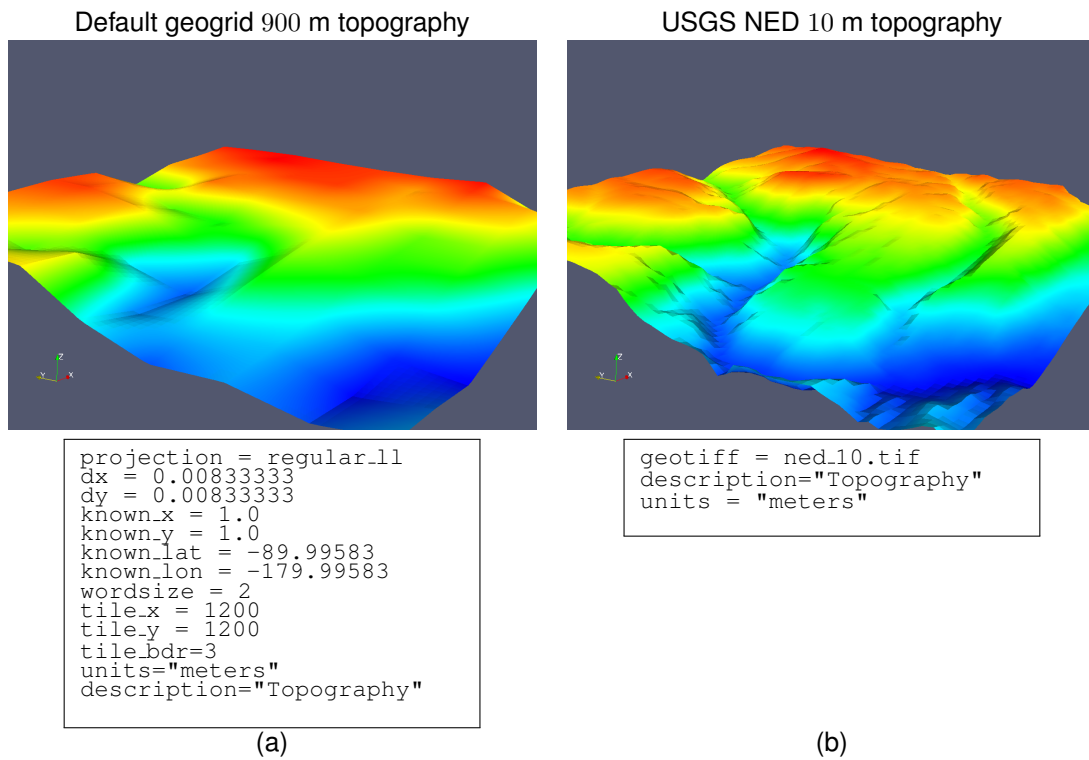
Figure 3: Comparing the topographical features in a 10 m resolution domain using the default geogrid dataset (a) and high resolution data from the USGS (b). The metadata needed in the index file is given below the images. For GeoTIFF datasets, the projection and geolocation information is determined automatically from the GeoTIFF metadata.
