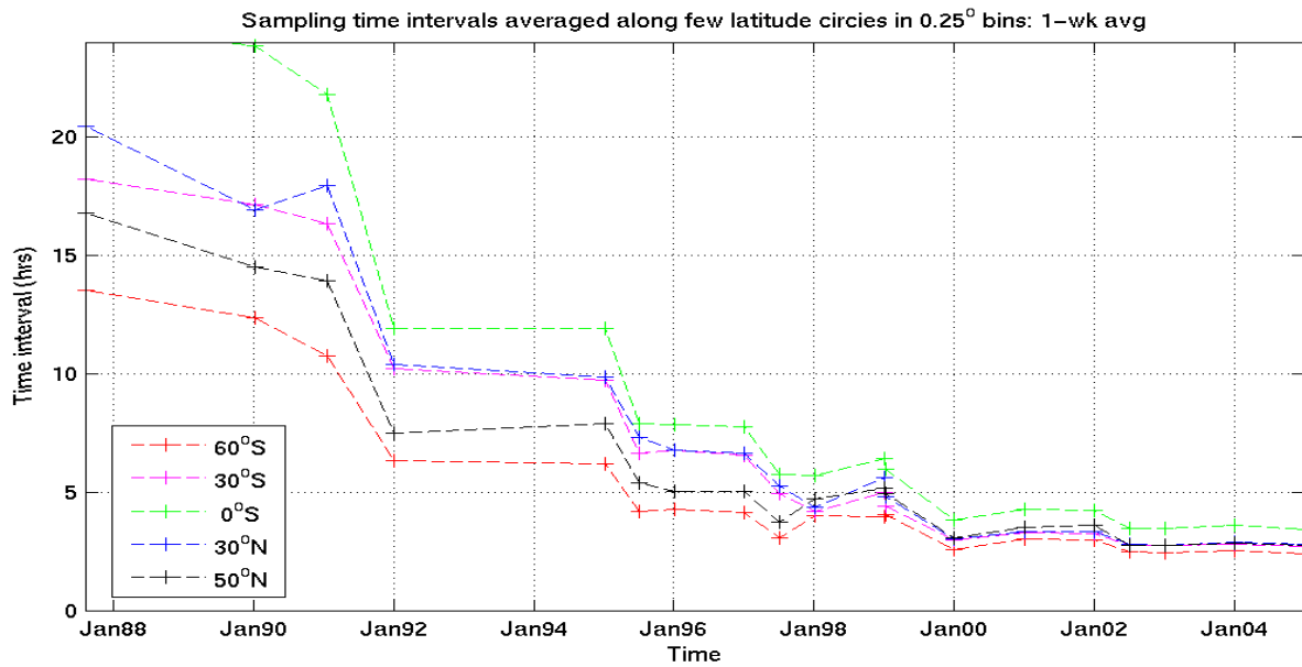
Figure 4: Sampling time intervals in the 0.25^\circ bins. Shown are zonal averages along 5 latitude circles and averaged over 1 week.
