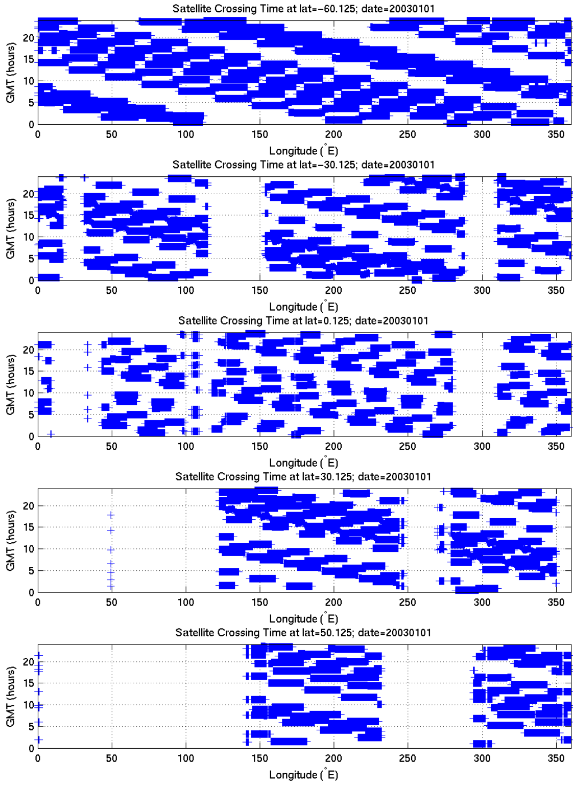
Figure 2a: Satellite passing times along 5 latitude circles for 1 January 2003. Data bin grids are 0.25° in space.
