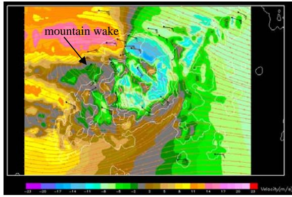
Figure 6 Surface (wind barbs) and 50-m winds (streamlines and velocities resolved along the LIDAR's radials) at the time of the largest mountain wake west of HKIA in the horizontally-homogeneous initialization run based on the vertical profiles in Figure 5
