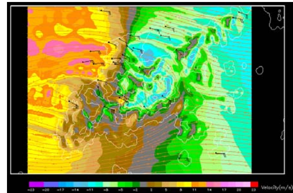
Figure 8 Same as Figure 6, but for large U , small \Delta\theta and large D
