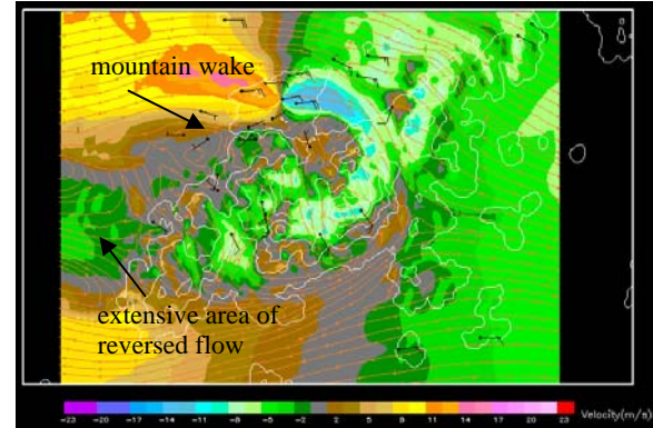
Figure 7 Same as Figure 6, but for small U , large \Delta\theta and small D
