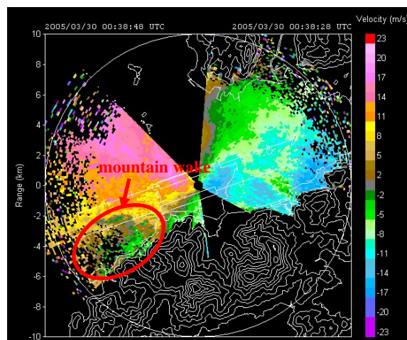
Figure 4 LIDAR's radial velocity imagery at 8:38 a.m., 30 March 2005.
