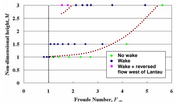
Figure 9 Regime diagram ( M \times F_\infty ) for Lantau Island simulations and regime boundaries (brown dotted lines).
