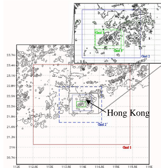
Figure 2 Domains of the nested model grids: solid and broken lines refer to the domains in the forecasting mode (Grids 1, 2 and 3) and the horizontally-homogeneous initialization simulations (Grids 2' and 3') respectively.
