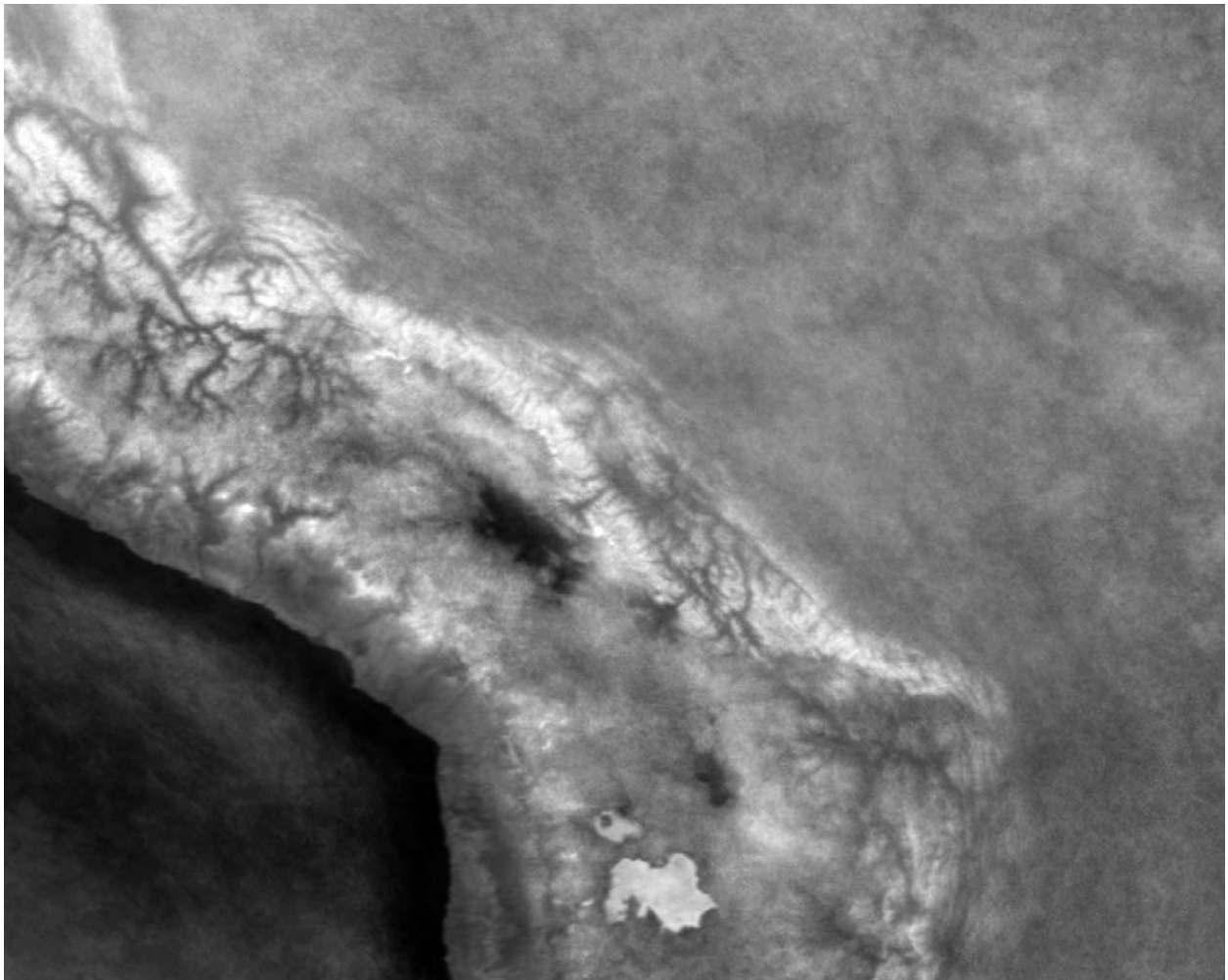
Fig. 3. Average of Dec-Feb GOES visible images at 1745 UTC for the year 2004-5. Note that Lake Titicaca is dark (minimum cloudiness), most canyons are dark (low cloudiness). Other features include the large and highly reflective Salar de Uyuni near the bottom (dry lake), and the region of less stratocumulus along and off the coast of Peru and Chile.
