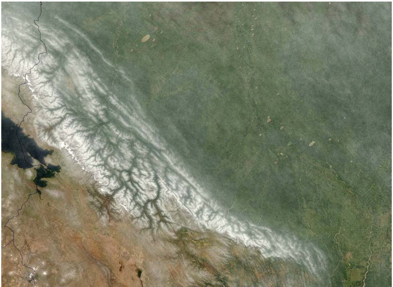
Fig. 5. The average of the two images shown in Fig 4. Some enhancements have been made (contrast/saturation changes).
