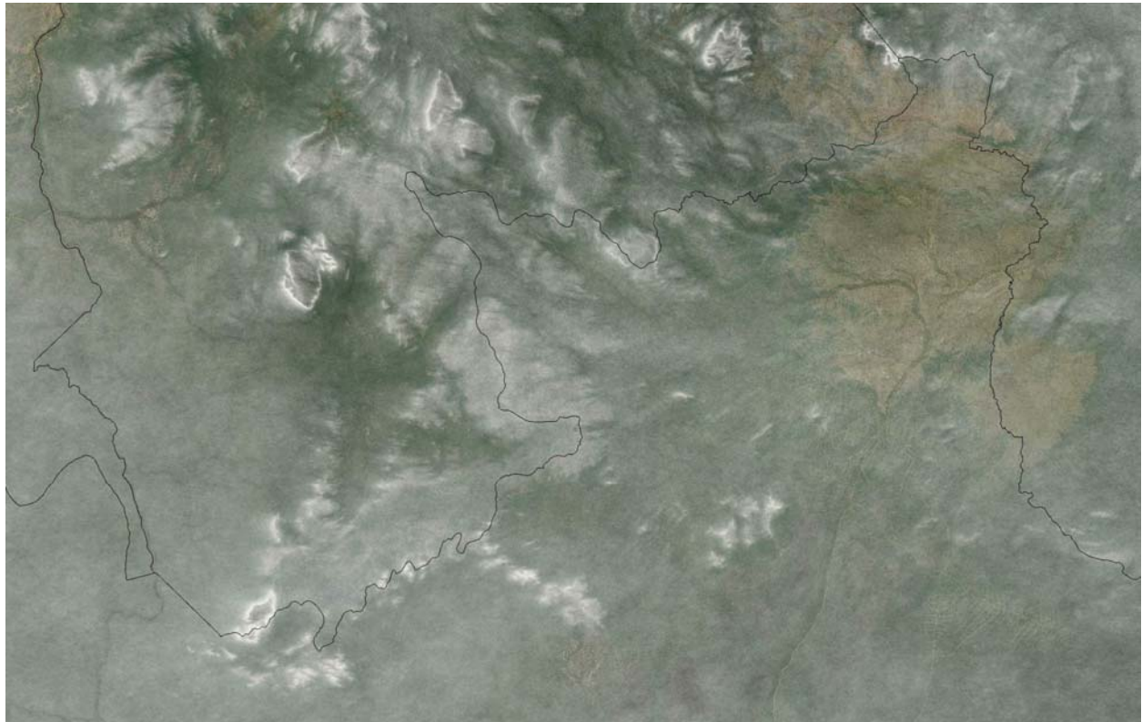
Fig. 6. The region of far southern Venezuela and extreme northern Brazil (centered around 3°N, 63°W). The cloudiness is a maximum over higher peaks and the edges of the Tepui's – elevated sandstone plateaus. Cloudiness is clearly a maximum at the edges of these plateaus (rather than on top), contrasting with normal peaks, where cloudiness is more closely centered about the peak. Distinctly less cloudiness (darker green areas) is evident between the higher terrain features. Rivers are darker – less cumulus development over the cooler surface.
