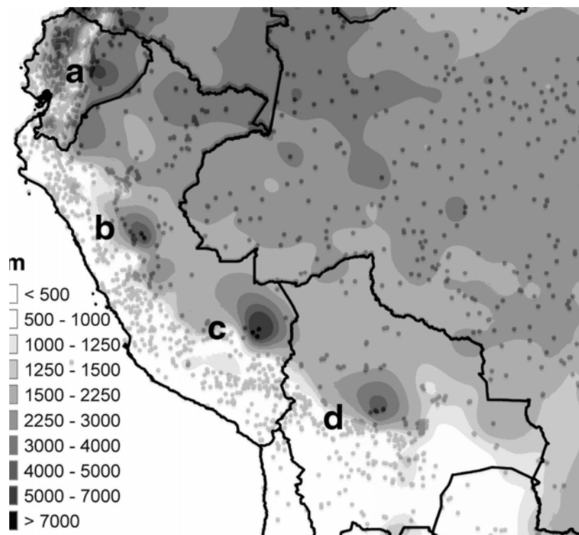
Fig. 1. Annual rainfall from WorldClim data base. Locations of raingauges entering the analysis are shown. The maxima in rainfall on the Andean east slopes is not well-defined because of a lack of raingauges.
