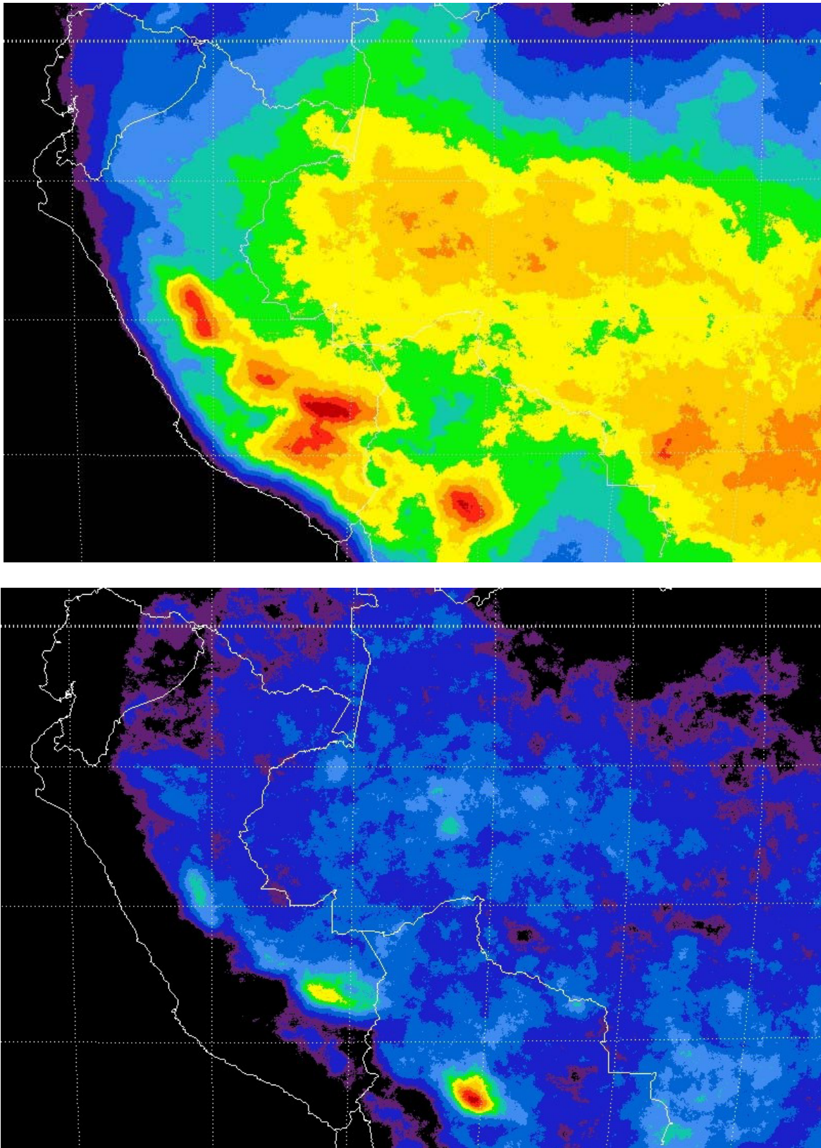
Fig. 2. Frequency of clouds colder than -38^{\circ}\text{C} (above) and -65^{\circ}\text{C} (below), averaged over the months of Dec-Feb for the years 2004-5 (Southern Hemisphere summer). Red is highest frequency, black (zero) lowest. Note the small geographical extent of the maxima.
