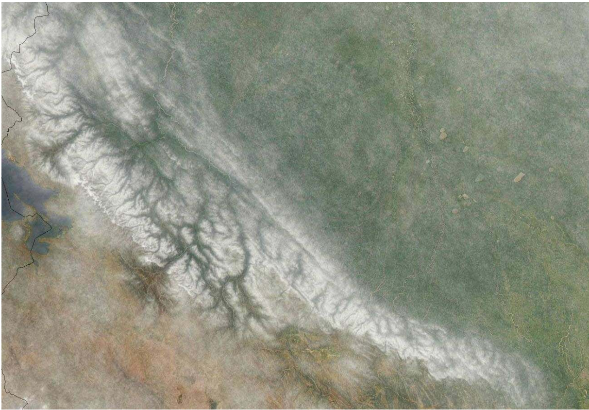
Fig. 4. Terra composite (above) (~1310 UTC) and Aqua composite (below) (~1740 UTC). Each composite used 60 images. Note more diffuse nature of cloudiness in Aqua composite.
