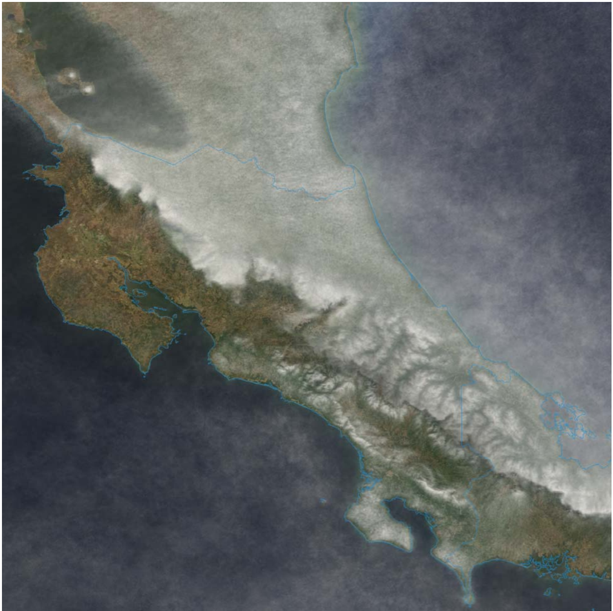
Fig. 7. Costa Rica and part of southern Nicaragua and western Panama. This composite is based on images from the dry season, Jan-March, 2004-5. During this period the trade winds are relatively strong from the east and the Pacific side of Central America is relatively cloud-free. The very sharp boundary of the clouds over northern Costa Rica is apparent, as is the effect of canyons (valleys have less cloudiness) on the cloud cover over southeastern Costa Rica. High cloud amounts on the isolated volcanic peaks in Lake Nicaragua are also evident.
