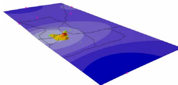
Figure 7: Comparison of interpolated surfaces of PSD and continuous monitor ozone data. PSD data typically shows peaks in the central city area that are not shown in the continuous monitor results. Continuous monitors are shown in pink, visible PSD sites are shown in green.
