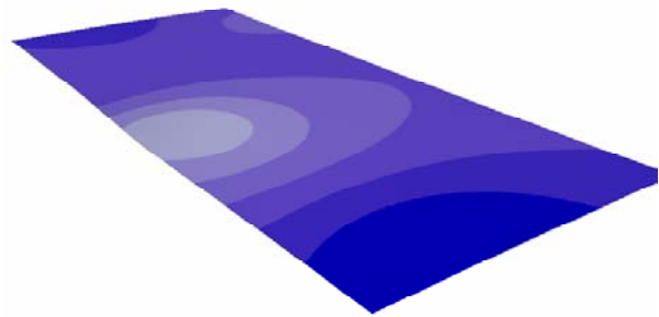
Figure 6: Three-dimensional model of the interpolated surface for the continuous monitor ozone data for Week 5. The contour color scale is the same as in Figure 4.
