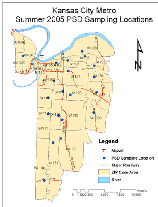
Figure 1: Sampling locations for the 2005 GLO project passive ozone sensors.
