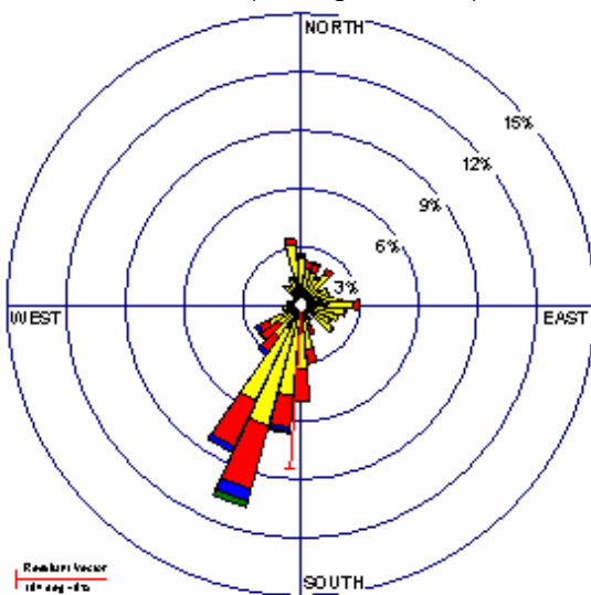
Figure 8: Windrose for Kansas City Downtown Airport. Windspeed color scale is in increments of 2.5 m/s. Yellow is the 2.5 to 5.0 m/s bin.
