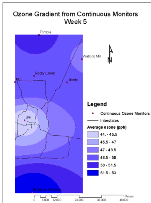
Figure 4: Weekly average ozone concentration gradient from continuous monitors.
