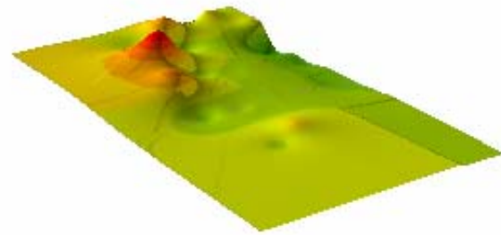
Figure 5: Three-dimensional model of the interpolated surface for the PSD ozone data for Week 5. The contour color scale is the same as Figure 3.
