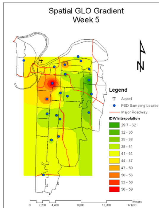
Figure 3: Representative IDW interpolation of spatial distribution of GLO based on PSD data. Week 5 coincided with two eight-hour ozone standard exceedences.
