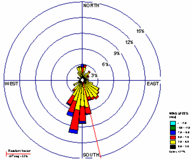
Figure 9: Windrose for KCI airport. Windspeed color scale is in increments of 2.5 m/s.
