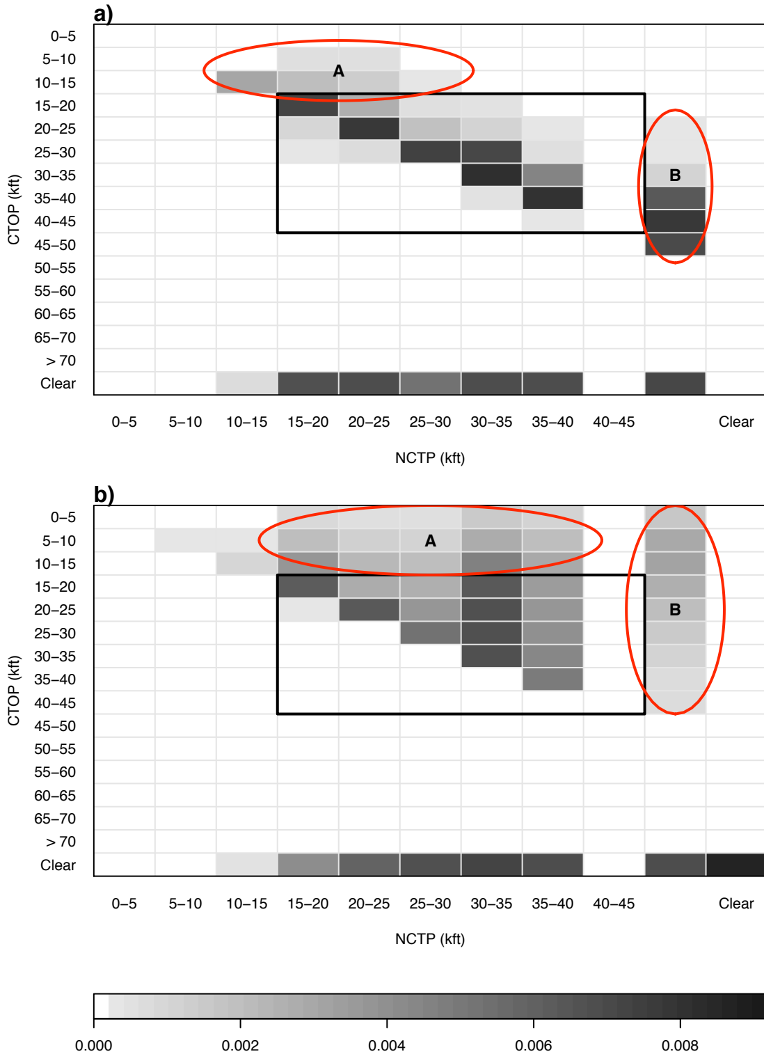
Figure 5. Joint Probability Distributions for CTOP and NCTP. Results are presented for (a) opaque (ECA \geq 95\% ) and (b) non-opaque (ECA < 95\% ) clouds. The ellipses labeled 'A' in figures 5.5 (a) and (b) roughly designate the comparisons excluded by the measures-oriented statistics because the CTOP value was below the valid range of the algorithm.
