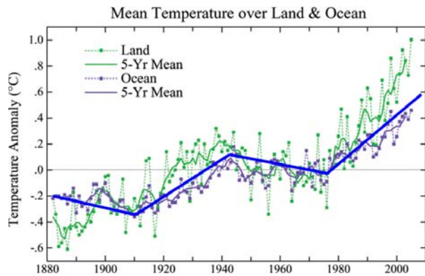
Figure 5. Change in global land and ocean temperature anomaly over the last 125 years.
