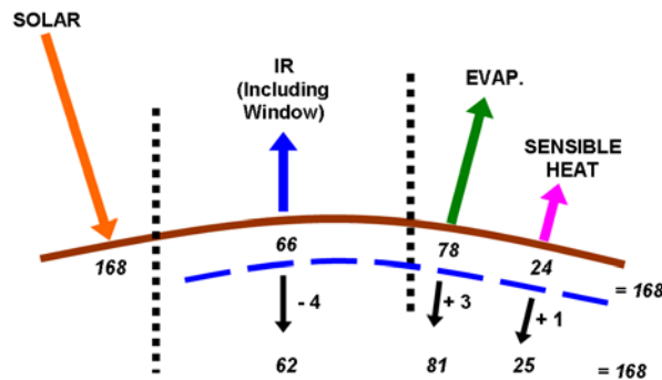
Figure 7. Global mean surface energy budget ( w/m^2 ) and change with 2 \times CO_2 .
