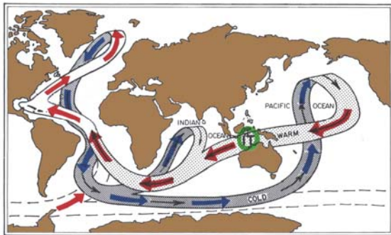
Figure 1. Idealized global ocean conveyor belt or THC.
