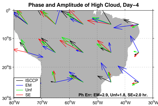
Figure 2: Phase and amplitude of the diurnal cycle of high cloud cover over the Amazon region from ISCCP and day-4 forecasts from the ensemble mean (EM), unified scheme (Unf) and the superensemble (SE) during 22–31 March 2000. A northward arrow represents a phase at 00 hours and eastward arrow represents a phase at 09 hours.
