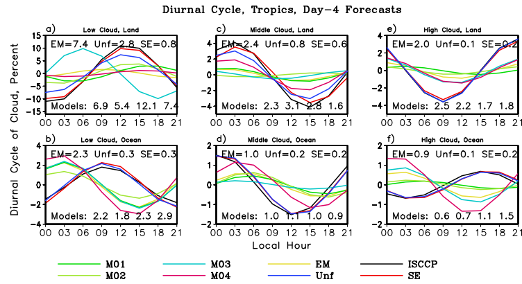
Figure 1: Diurnal cycle of low, middle and high cloud cover over the Tropics ( 0^{\circ} – 360^{\circ} E, 30^{\circ} S– 30^{\circ} N) from ISCCP and day-4 forecasts from the member models, ensemble mean (EM), unified scheme (Unified) and the superensemble (SE) during 22–31 March 2000. RMS error (in percent) of the total diurnal cycle for EM, Unified and SE are indicated at the top of the panels, and those for the member models are shown at the bottom of the panels.
