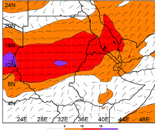
Fig. 1.3. ECMWF 3-day composite analysis of 600-hPa wind ( \text{m s}^{-1} ) for 27 July to 29 July 2000. Contours every 5 \text{m s}^{-1} .
