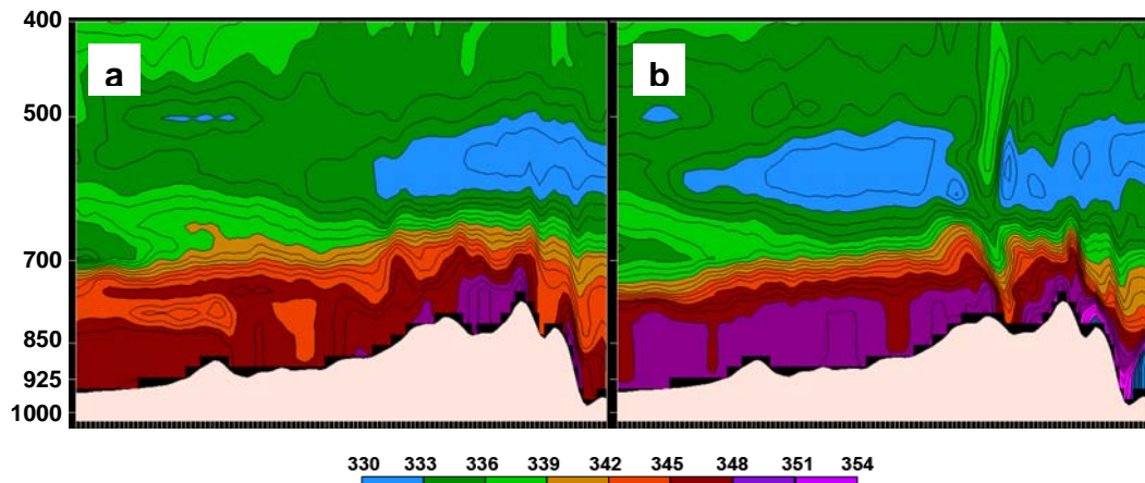
Fig. 3.4. MM5 4-km grid cross section of equivalent potential temperature (K) along 14.9^\circ\text{N} , and between 36.0^\circ\text{E} and 40.0^\circ\text{E} for a) 0900 UTC 28 July 2000, and b) 1300 UTC 28 July 2000. Contours are every 1 K, and shaded every 3 K.
