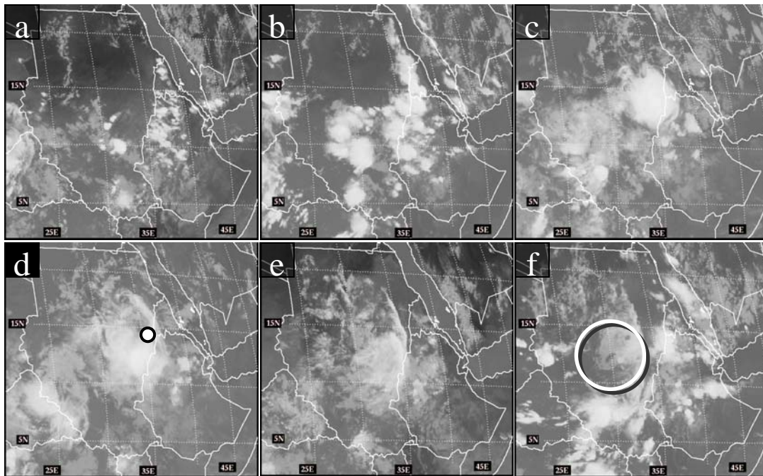
Fig. 1.1. METEOSAT-7 infrared-wavelength imagery for a) 1200 UTC 28 July 2000, b) 1600 UTC 28 July 2000, c) 2200 UTC 28 July 2000, d) 0400 UTC 29 July 2000, e) 1000 UTC 29 July 2000, and f) 1600 UTC 29 July 2000. Dot in d) depicts previous MCC center of c). Circle in f) encompasses visible MV. Imagery provided by EUMETSAT © 2003.
