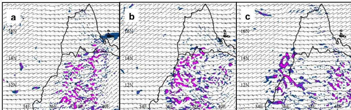
Fig. 3.2. MM5 4-km grid 600-hPa relative vorticity ( s^{-1} ) and wind ( m s^{-1} ) at a) 1200 UTC 28 July 2000, b) 1600 UTC 28 July 2000, and c) 2200 UTC 28 July 2000. Vorticity is shaded every 10^{-4} s^{-1} up to 4 \times 10^{-4} s^{-1} .
