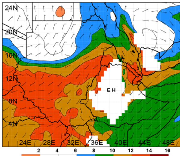
Fig. 1.2. ECMWF 3-day composite analysis of 850-hPa water vapor mixing ratio ( \text{g kg}^{-1} ) and wind ( \text{m s}^{-1} ) for 27 July to 29 July 2000. Contours every 2 \text{g kg}^{-1} .
