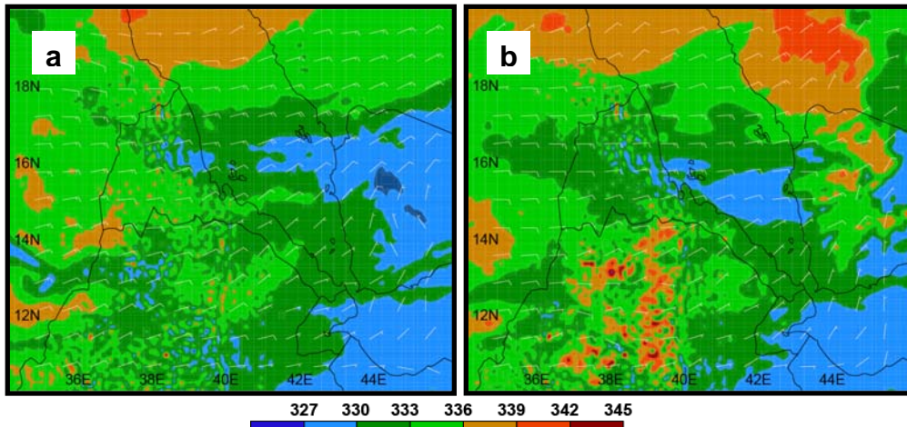
Fig. 3.3. MM5 12-km grid 550-hPa equivalent potential temperature (K) and wind ( \text{m s}^{-1} ) at a) 0600 UTC 28 July 2000, and b) 1200 UTC 28 July 2000. Equivalent potential temperature is shaded every 3 K.
