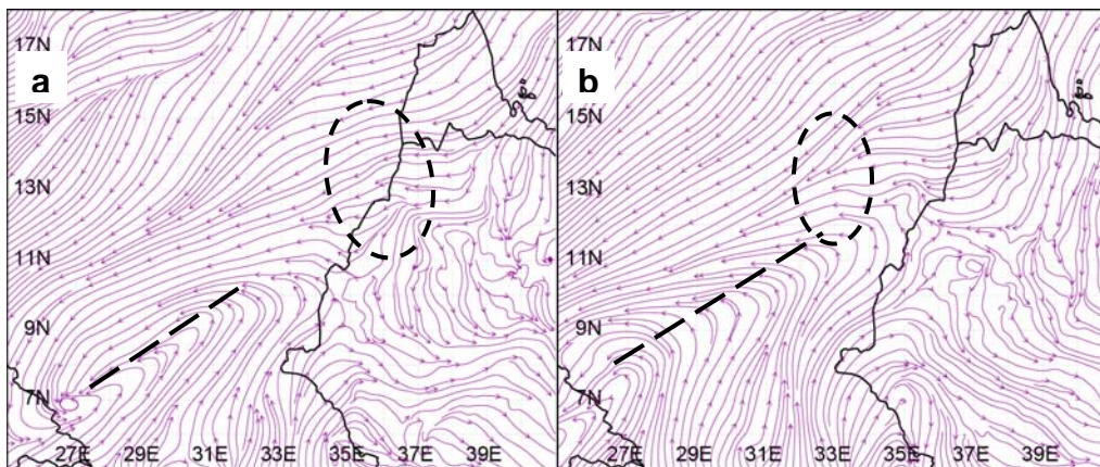
Fig. 3.5. MM5 12-km grid 700-hPa streamline field at a) 2200 UTC 28 July 2000, and b) 0600 UTC 29 July 2000. Dashed oval encircles signal of convective wave. Dashed line marks the apparent lee trough.
