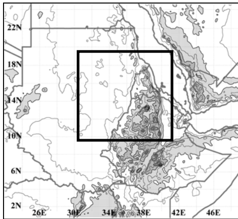
Fig. 2.1. GLOBE Project terrain (m) within the 12-km and 4-km spaced grids. Terrain is contoured every 500 m, and shaded every 1000 m above 1000 m.
