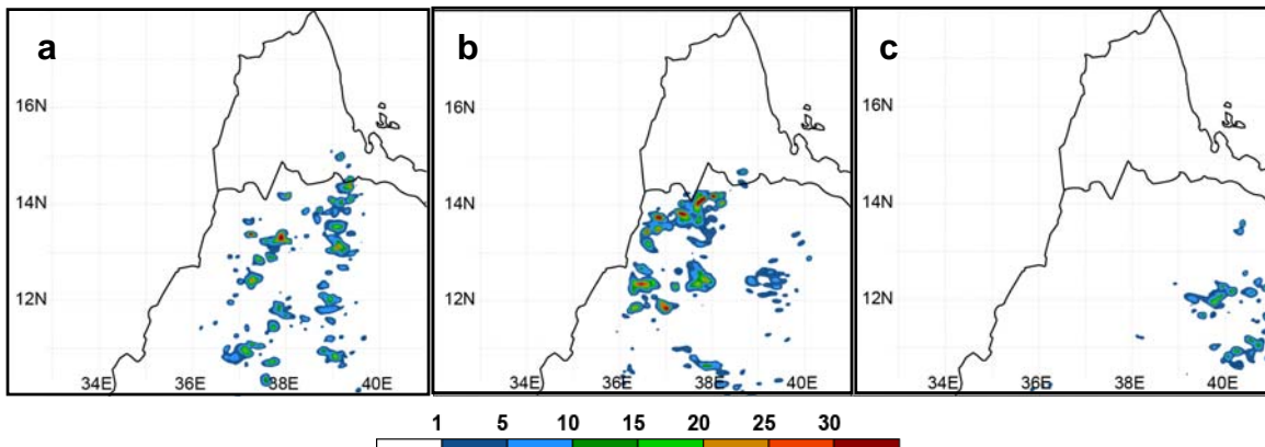
Fig. 3.1. MM5 4-km grid precipitation (mm) field simulated for a one-hour period ending at a) 1200 UTC 28 July 2000, b) 1600 UTC 28 July 2000, and c) 2200 UTC 28 July 2000.
