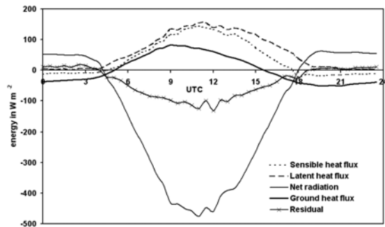
Figure 3: Mean diurnal cycle of all energy balance components for site A6 (maize) during the LITFASS-2003 period (Liebethal et al., 2006).
