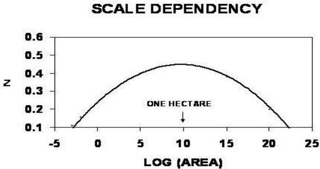
Figure 1. Scale dependence of the species-area relationship. The slope of the log species-log area curve, z , plotted against log (area).
