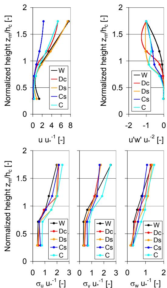
Figure 5: Representative profiles of measured turbulence statistics for the 5 exchange regimes: wind speed (a), vertical momentum flux, (b), standard deviation of alongwind (c), crosswind (d), and vertical wind (e). All values normalized with friction velocity. Figures (a) and (b) show AKIMA-interpolated profiles, (c) to (e) are linearly interpolated between measurement levels.
