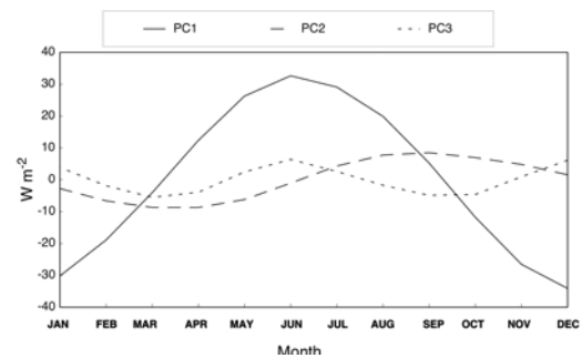
Figure 2: Principal components for downward shortwave flux at surface, Wm^{-2} .
