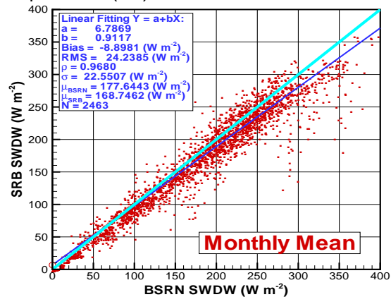
Figure 6: SRB(V2.6)-BSRN shortwave downward flux monthly mean comparisons.
