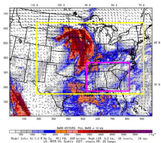
Figure 1. CAPE field valid at 2000 UTC from WRF run initialized at 00 UTC on 19 July 2006 also illustrating the domain used in the 00 UTC runs. The 12 UTC run domain is indicated by the yellow box. The magenta box depicts the area over which analyses were done.
