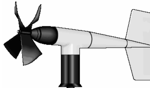
Figure 1. Schematic image of the propeller-and-vane type wind sensor used on the 5 KSC/CCAFS towers (R. M. Young Model 05305 Wind Monitor-AQ; see Computer Sciences Raytheon (2000) for details). Wind speed accuracy is +/- 0.58 kt. The starting threshold wind speed is 0.64 kt.
