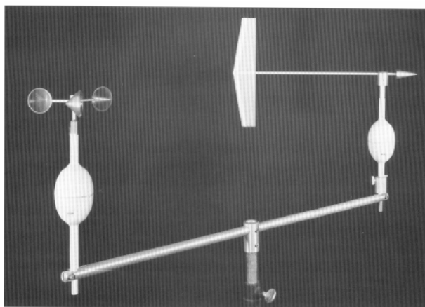
Figure 2. Image of the cup-and-vane type wind sensor mounted on the 5 VAFB towers used in this study (Met One Instruments Model TG1500 Wind Sensor System). Wind speed accuracy is \pm 0.15 kt or 1% of wind speed, whichever is greater. The distance constant is 5 ft.
